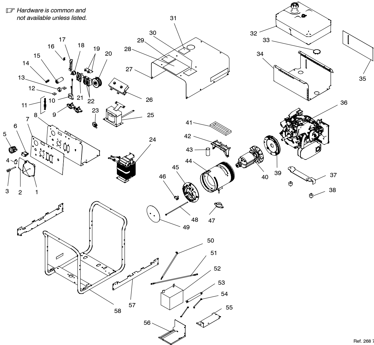
Figure 1-1. Main Assembly
