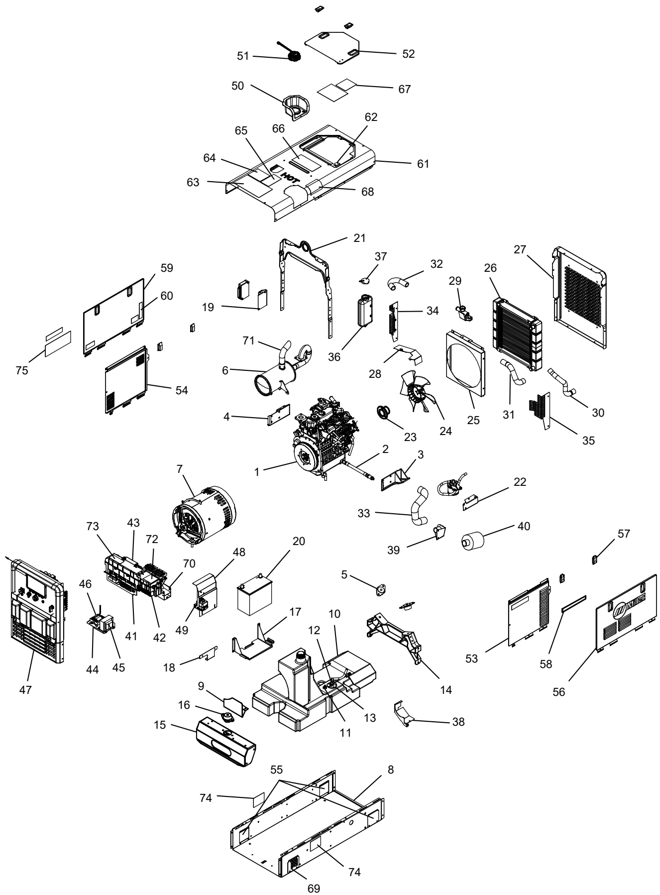
Main Assembly
