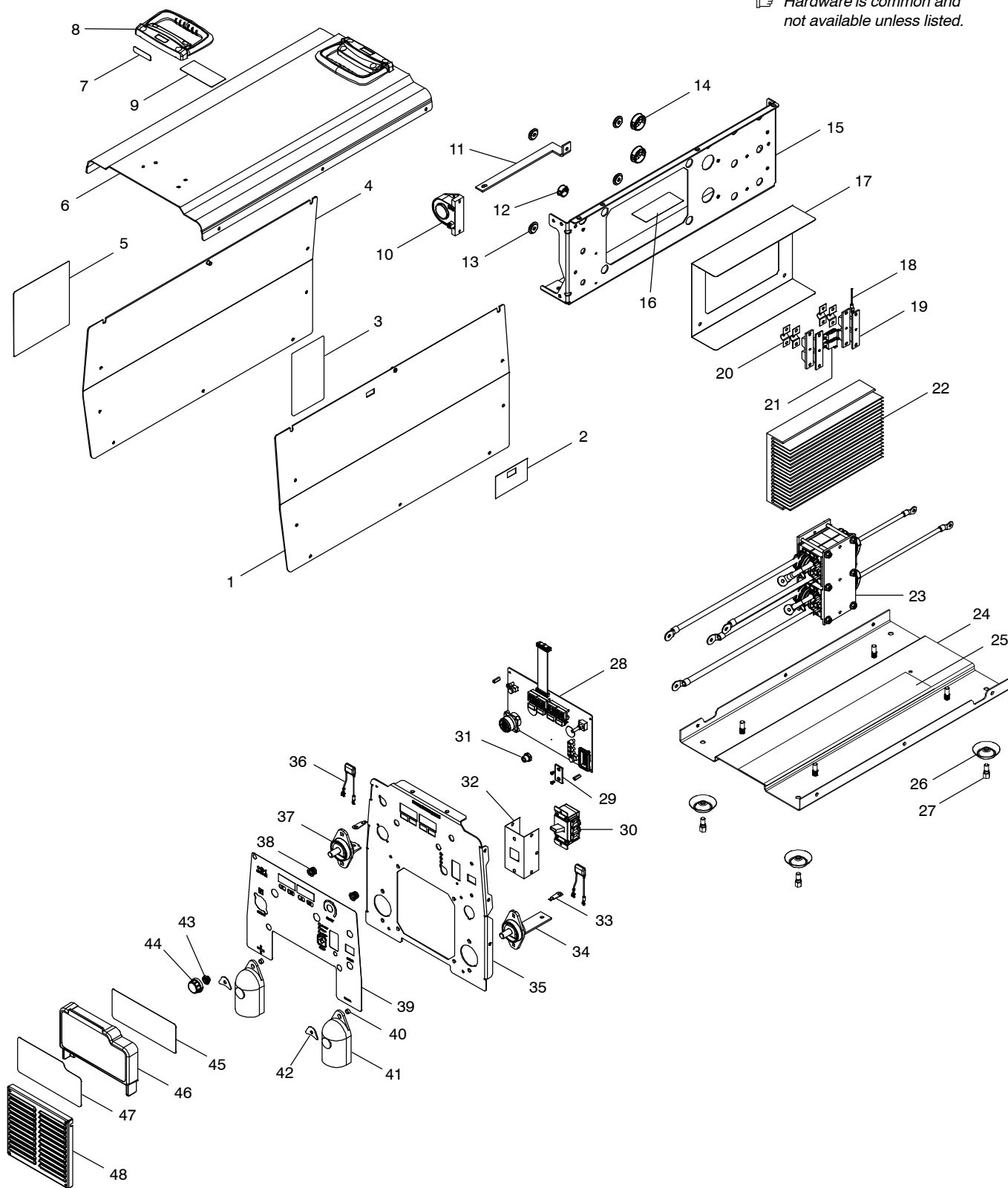
Figure 1-1. Parts Assembly
