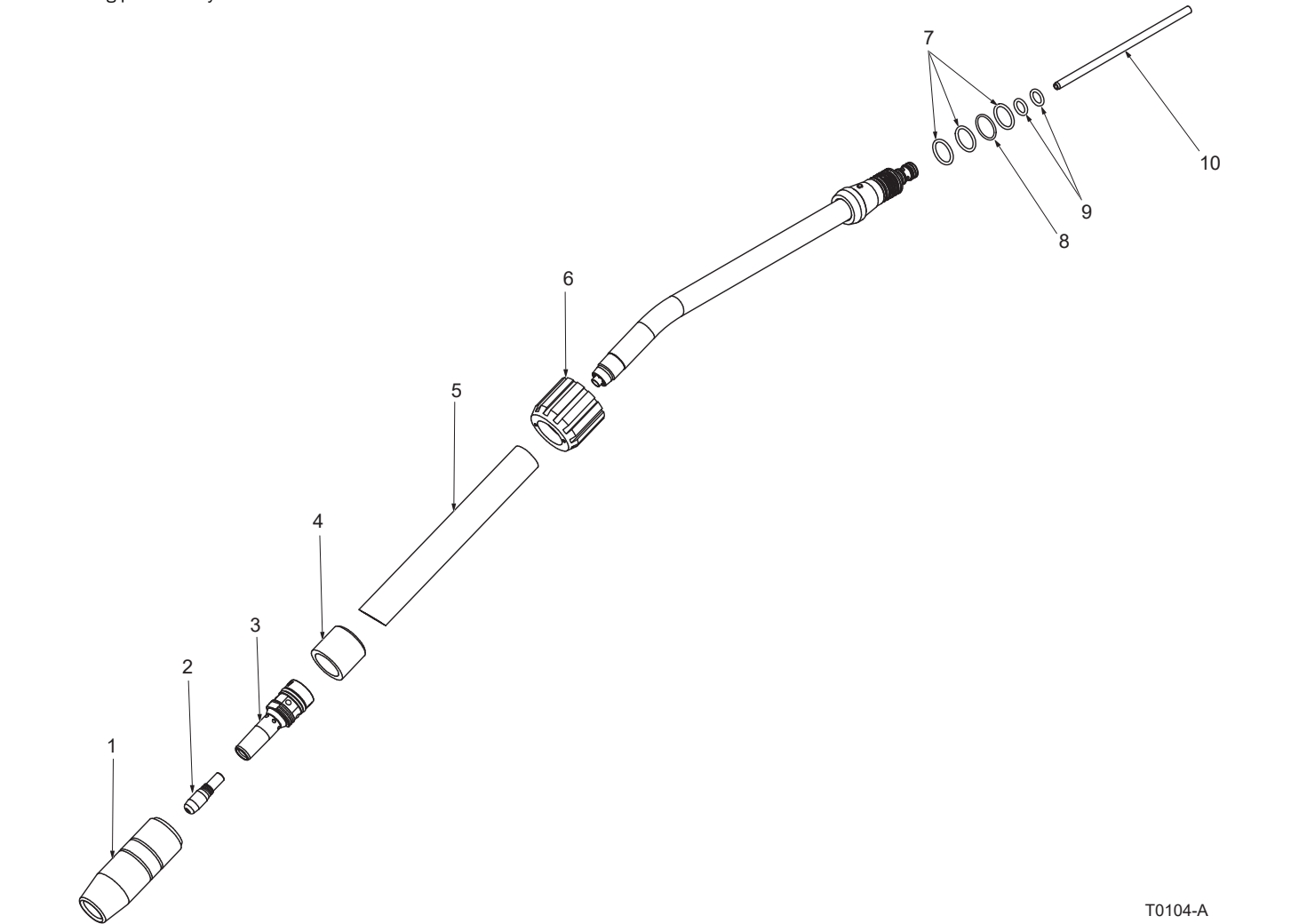
Water Head Tube Assembly
