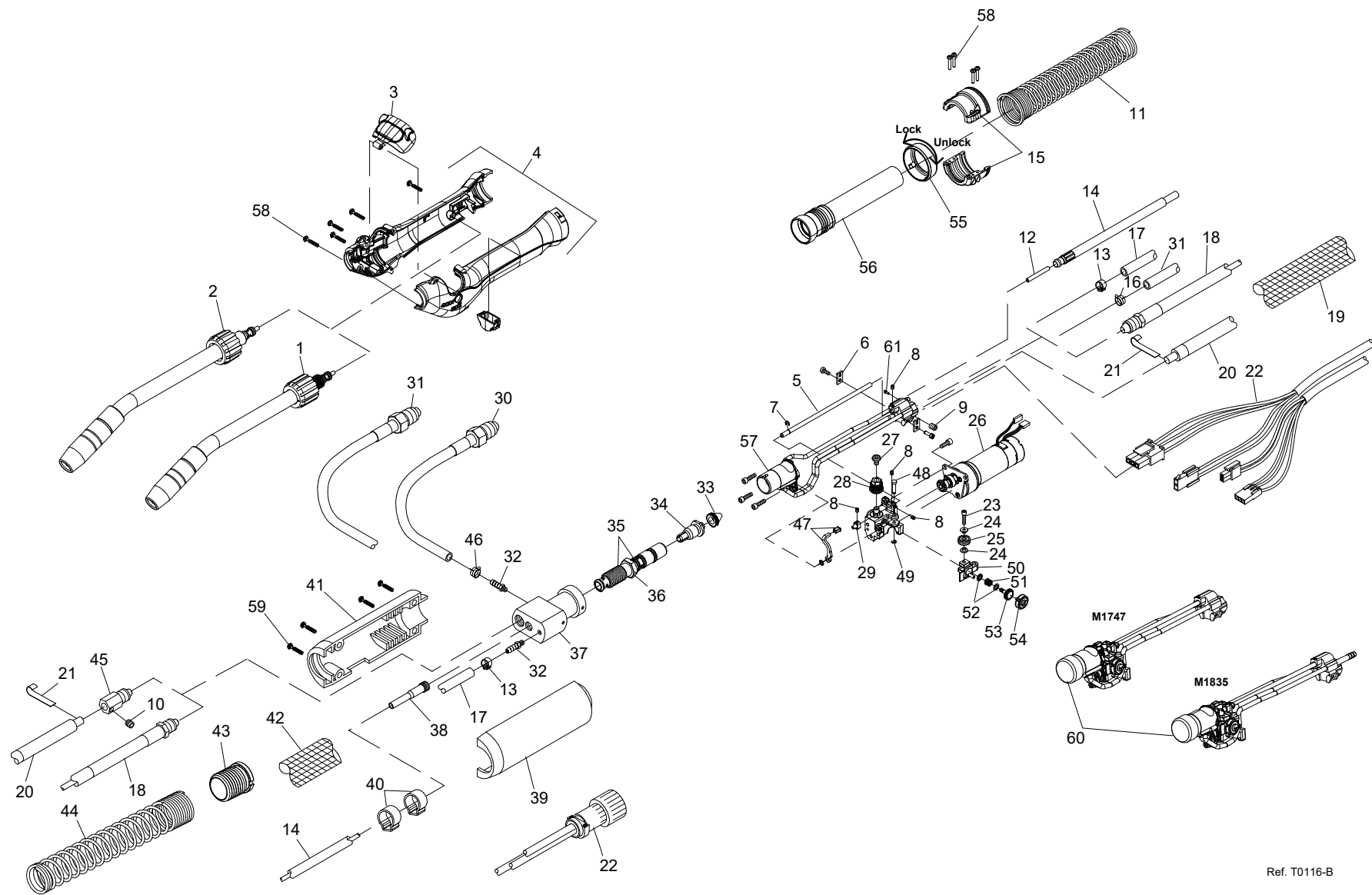
Main Assembly
