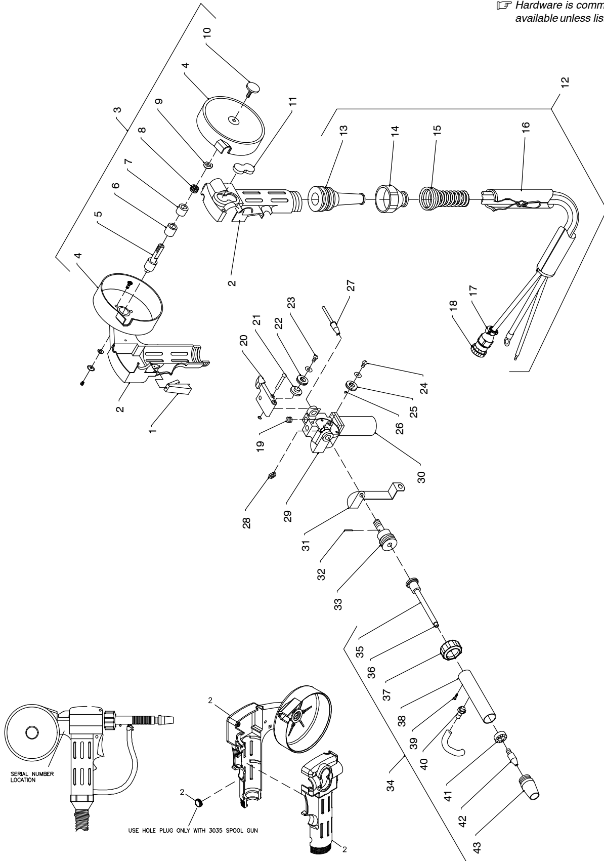
Figure 7-1. Complete Assembly For Spoolmate 3035
