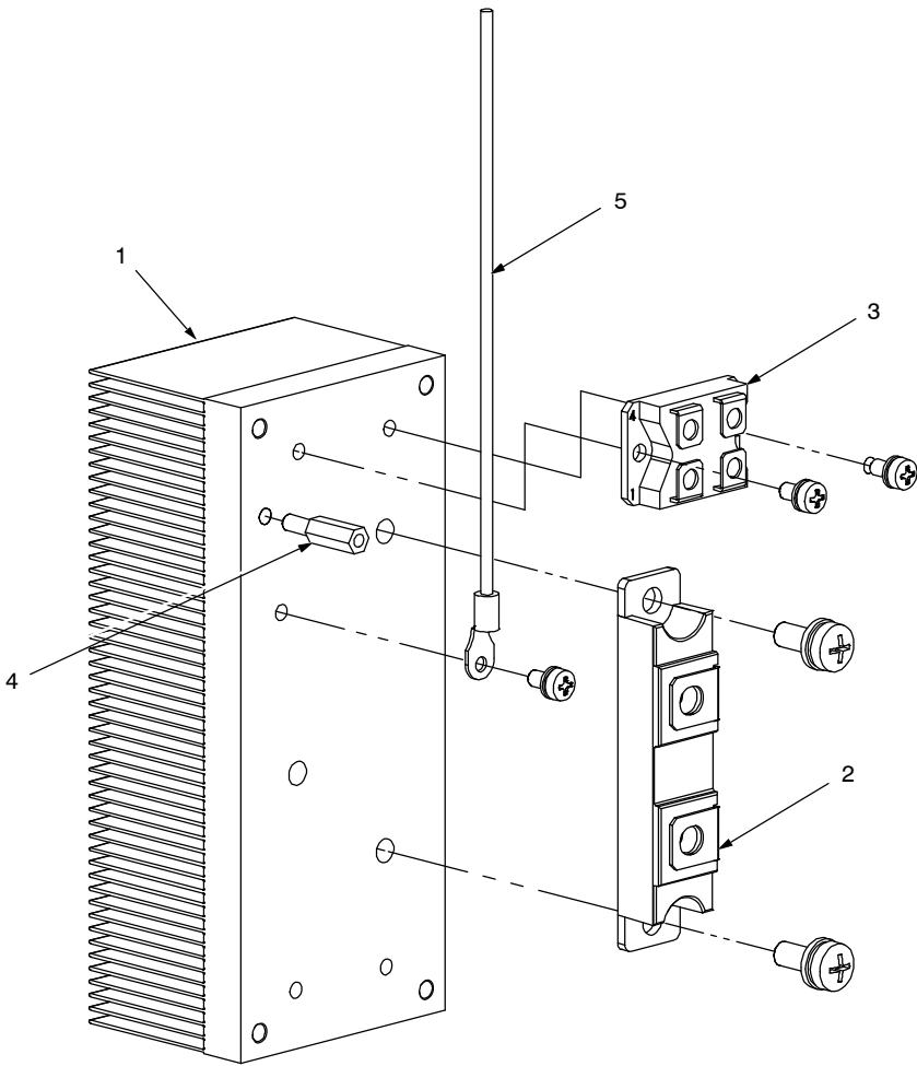
Figure 1-7. Diode Heat Sink Assembly (Maxstar 280)
