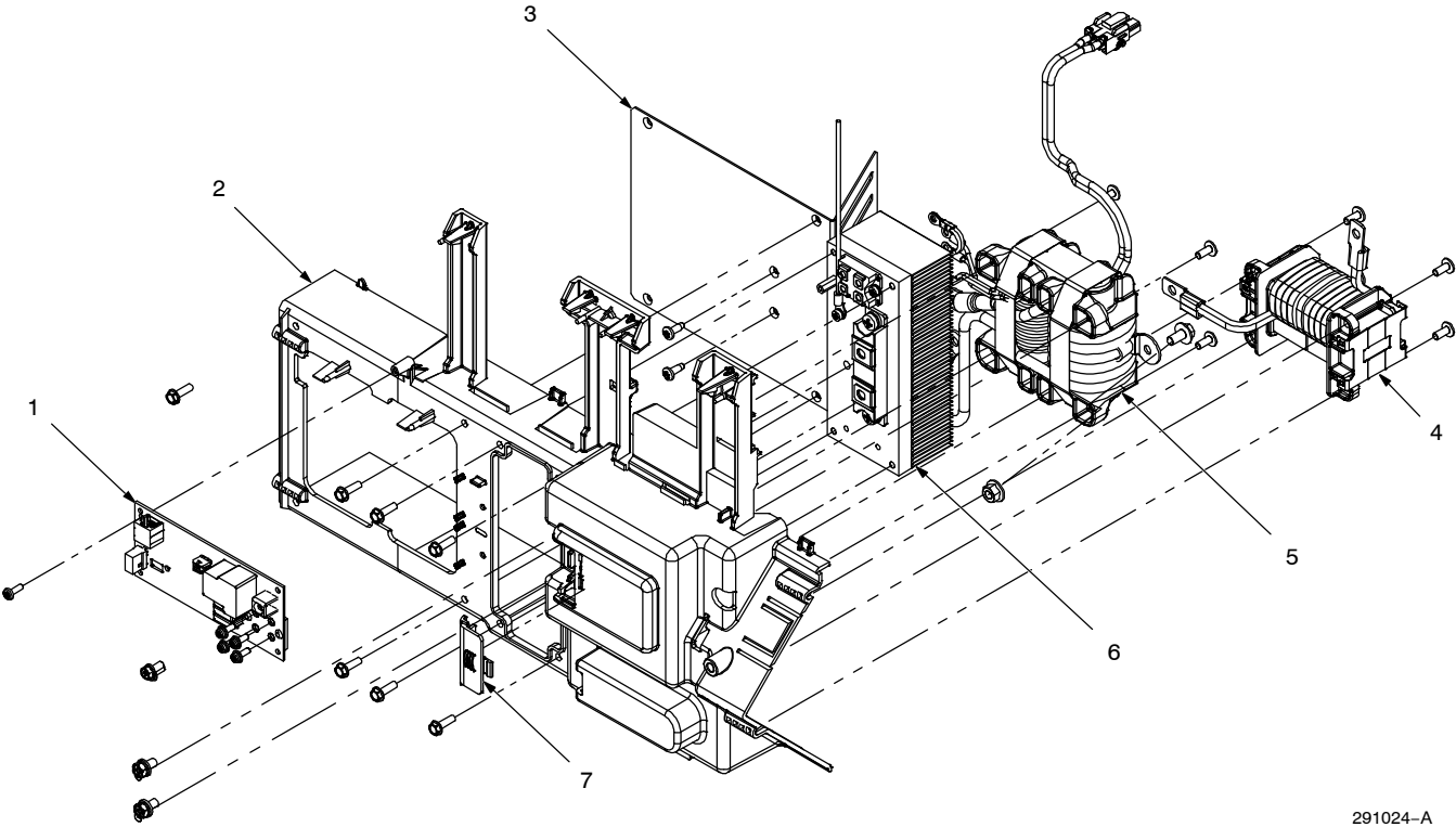
Figure 1-6. Maxstar 280 Wind Tunnel, Left Hand w/Components
