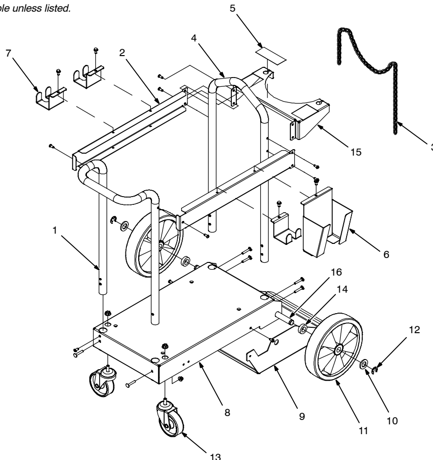
Figure 3-1. Complete Assembly For 254522
