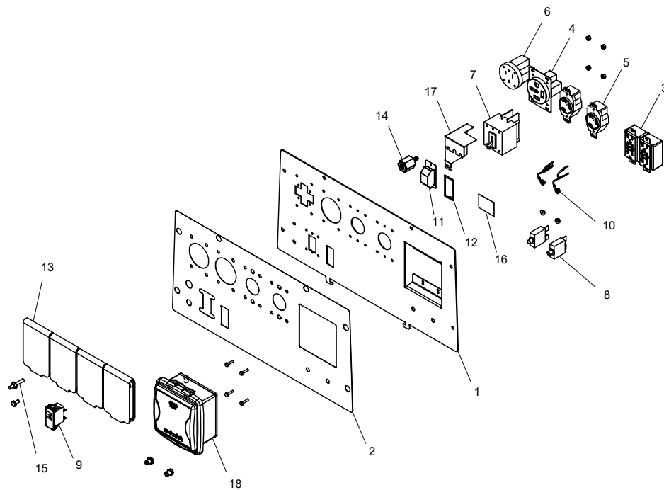
Auxiliary Power Panel, North America
