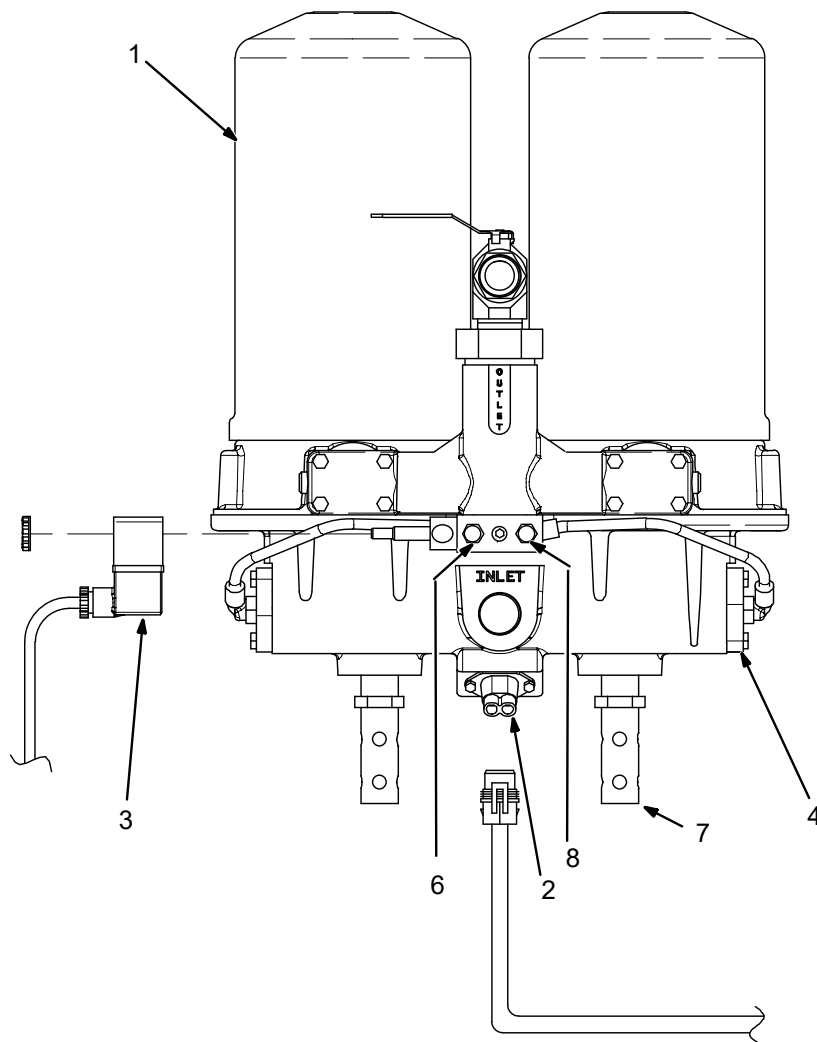
Optional Air Dryer Assemblies
