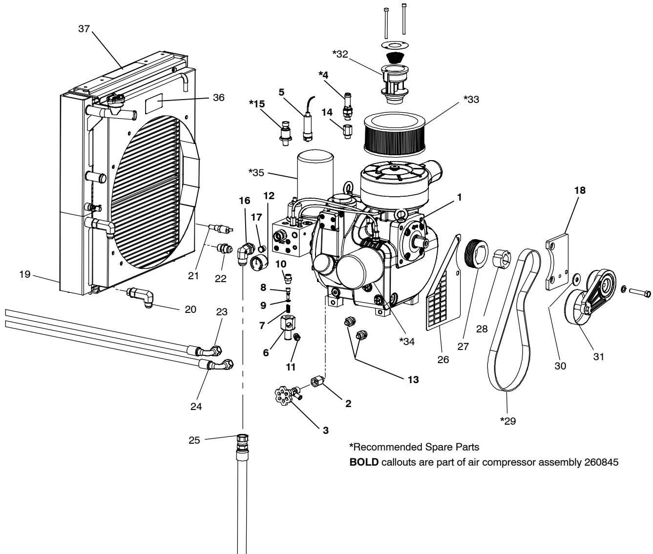
Figure 1-3. Air Compressor
