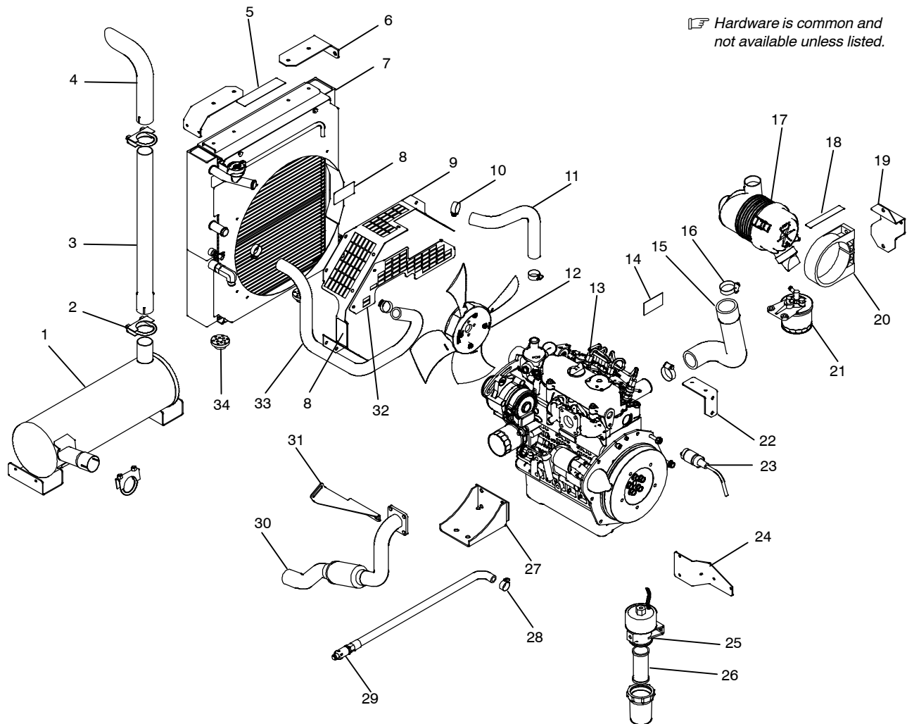
Figure 1-8. Engine
