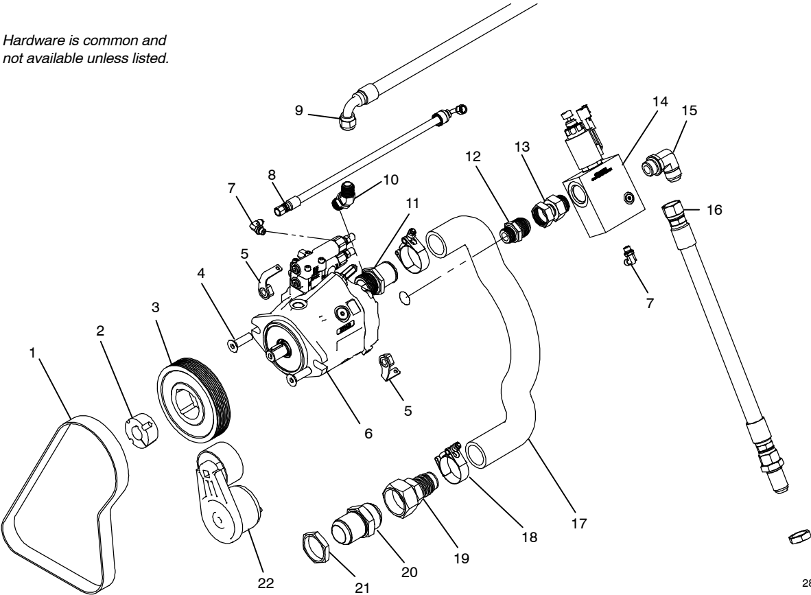
Figure 1-4. Hydraulic System Open Center (If Equipped)
