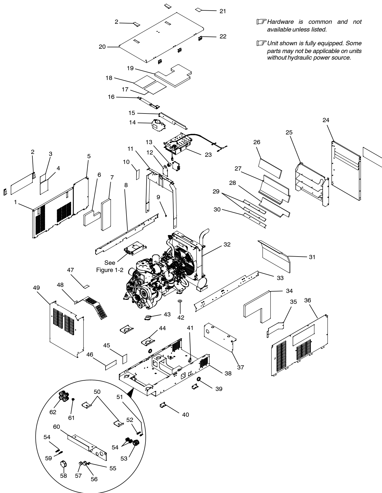
Figure 1-1. Main Assembly
