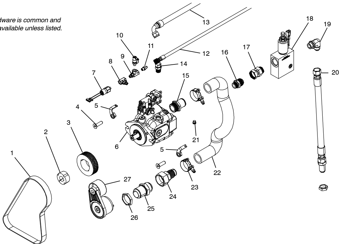
Figure 1-5. Hydraulic System Closed Center (If Equipped)
