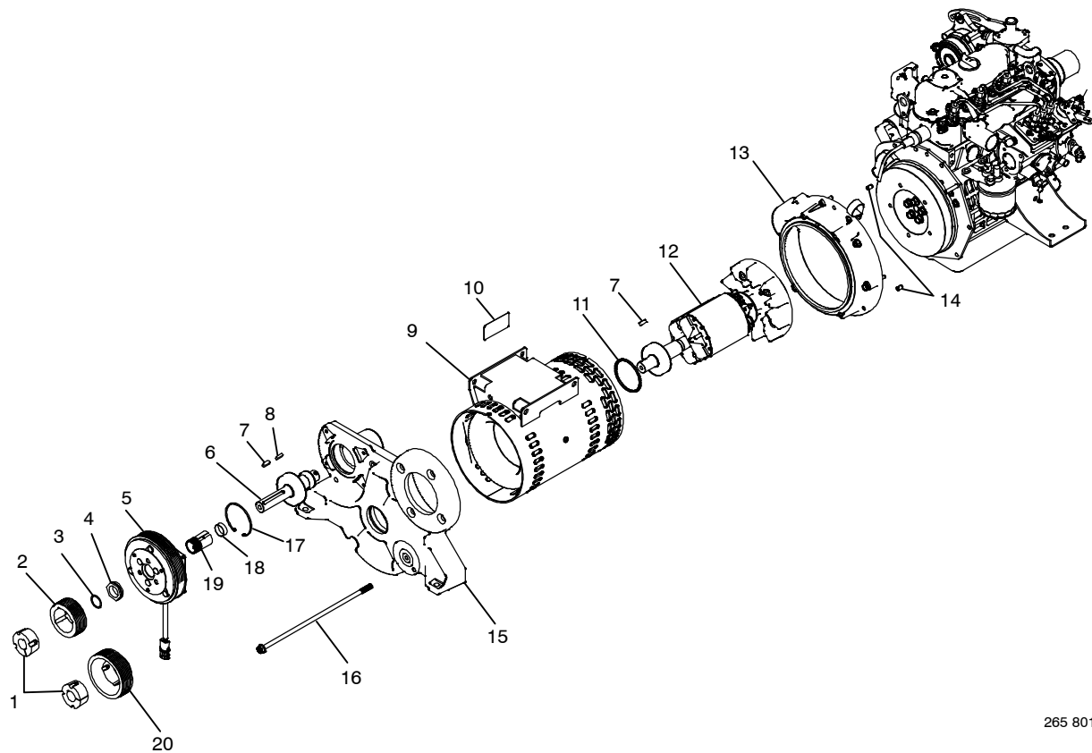
Figure 1-7. Generator Assembly
