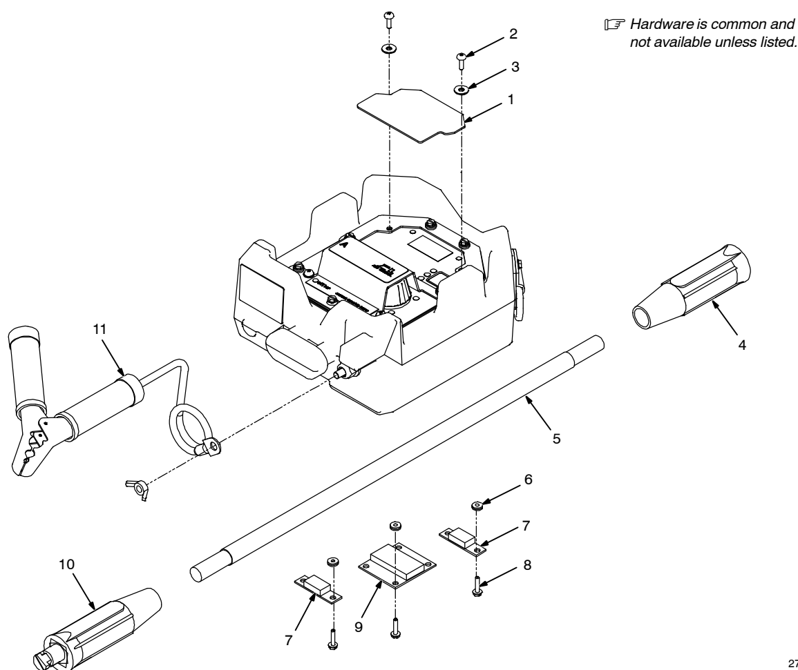
Figure 1-1. ArcReach Stick/TIG Remote Assembly
