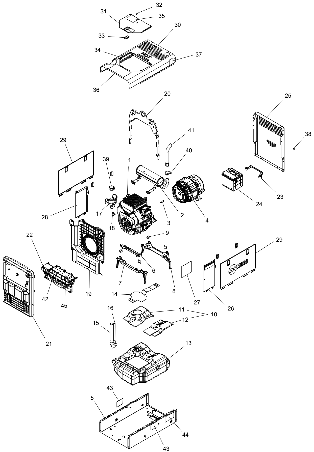
Main Assembly
