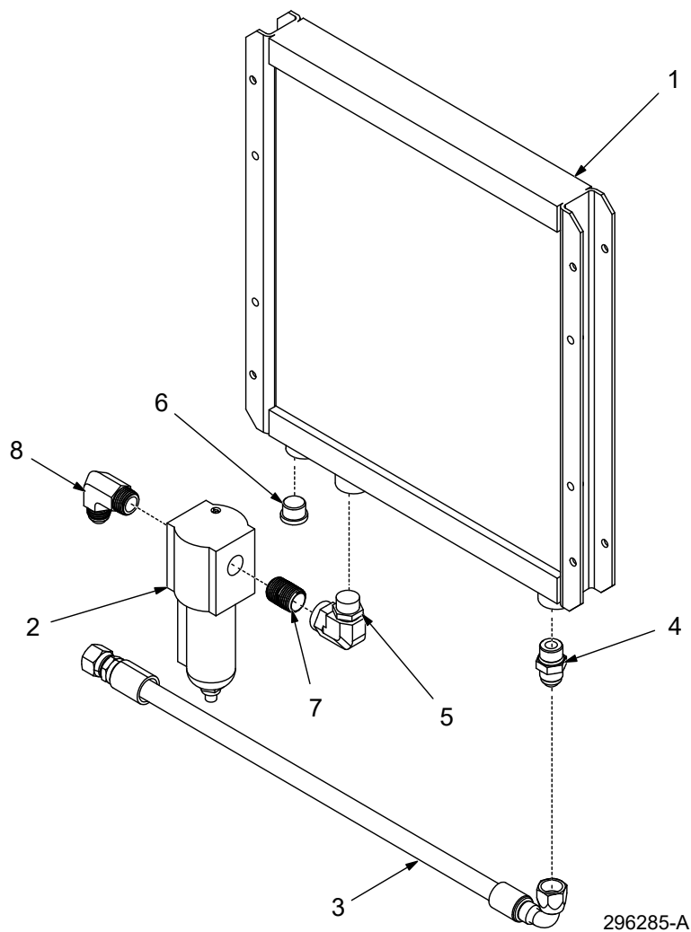
Air Cooler-Separator Assembly
