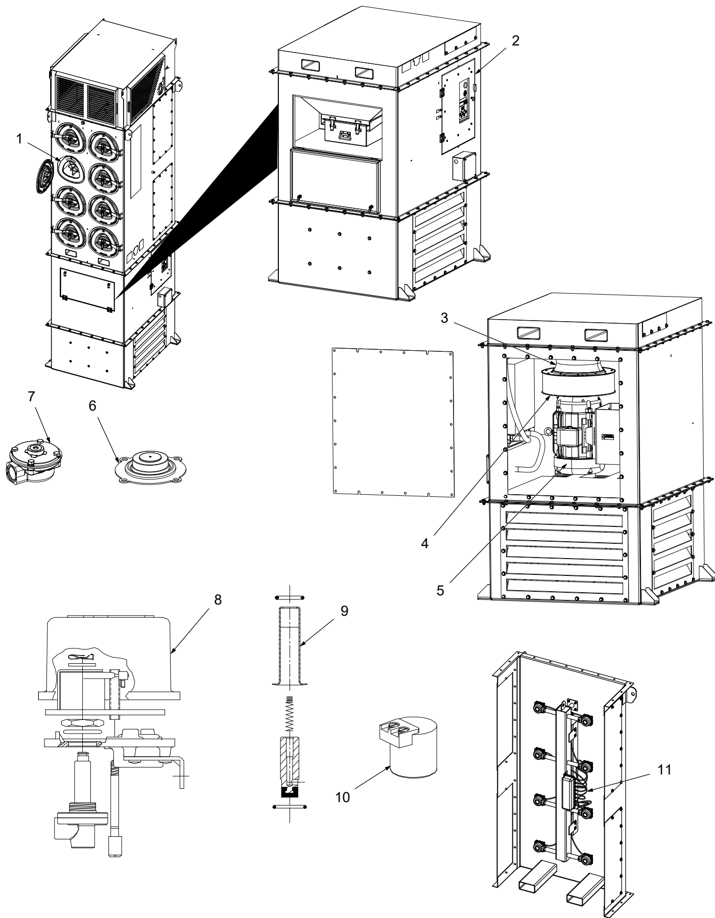
Parts Assembly
