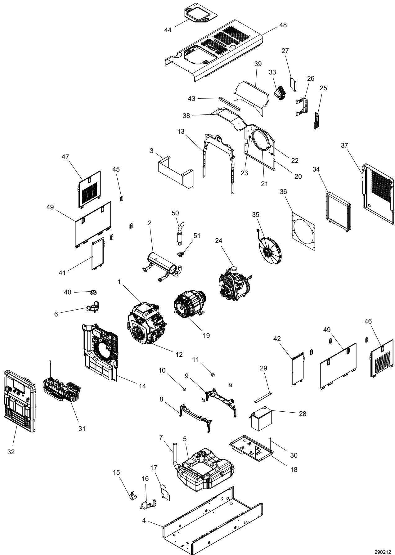
Main Assembly
