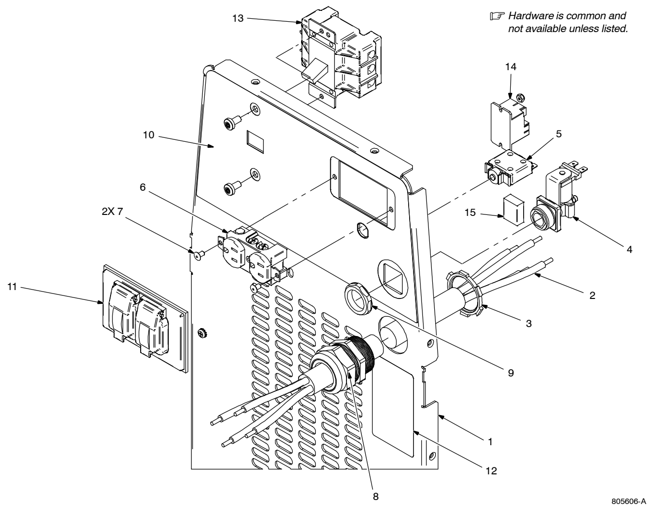
Figure 2-3. Panel, Rear w/Components
