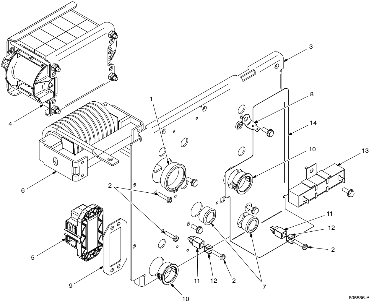
Figure 1-6. Wind Tunnel, Left Hand w/Components
