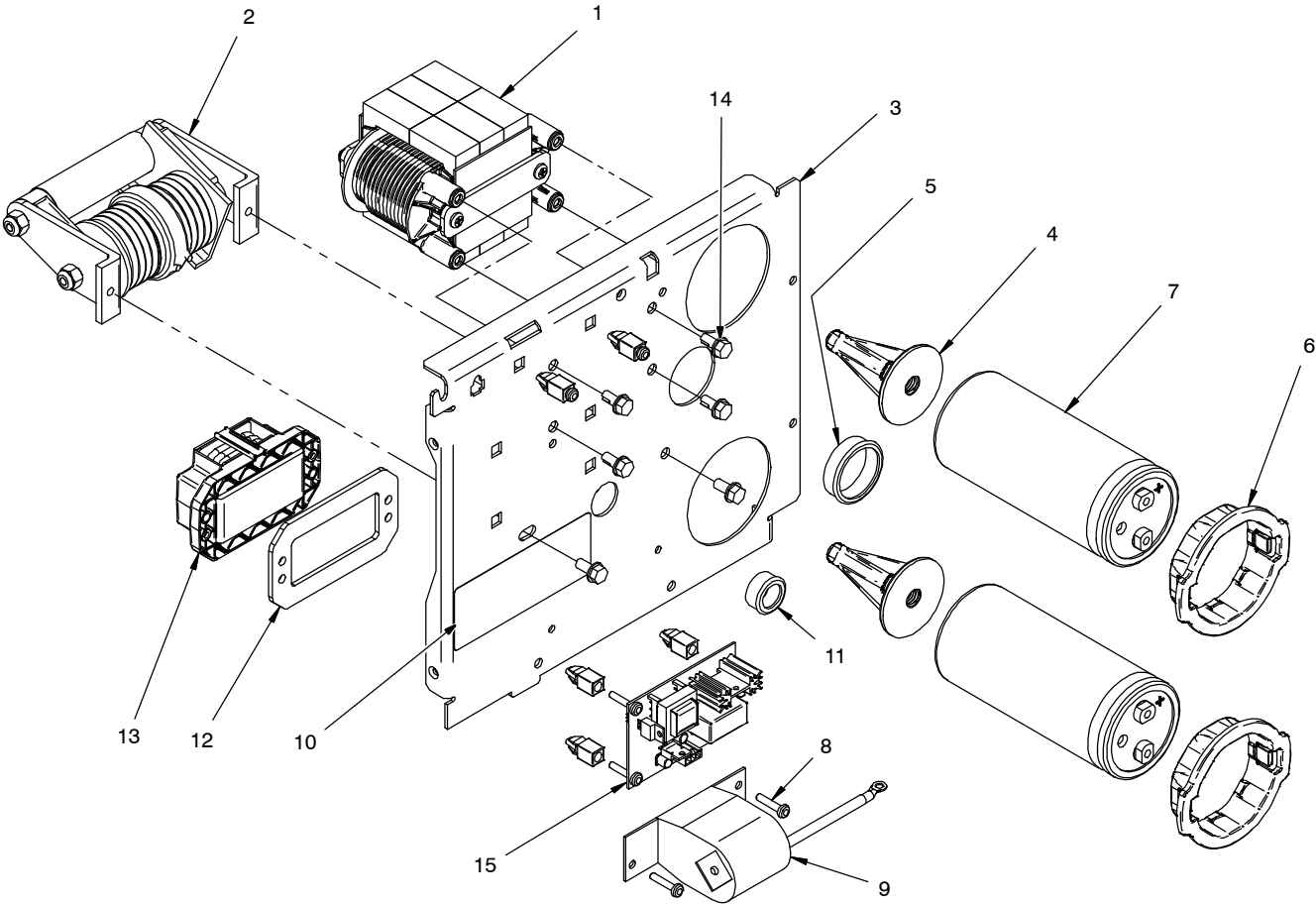
Figure 2-4. Wind Tunnel, Right Hand w/Components
