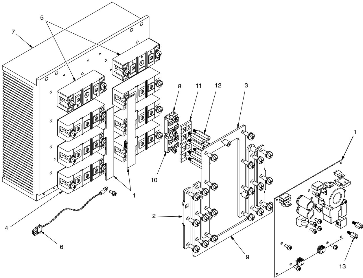
Figure 1-7. Heatsink, Secondary
