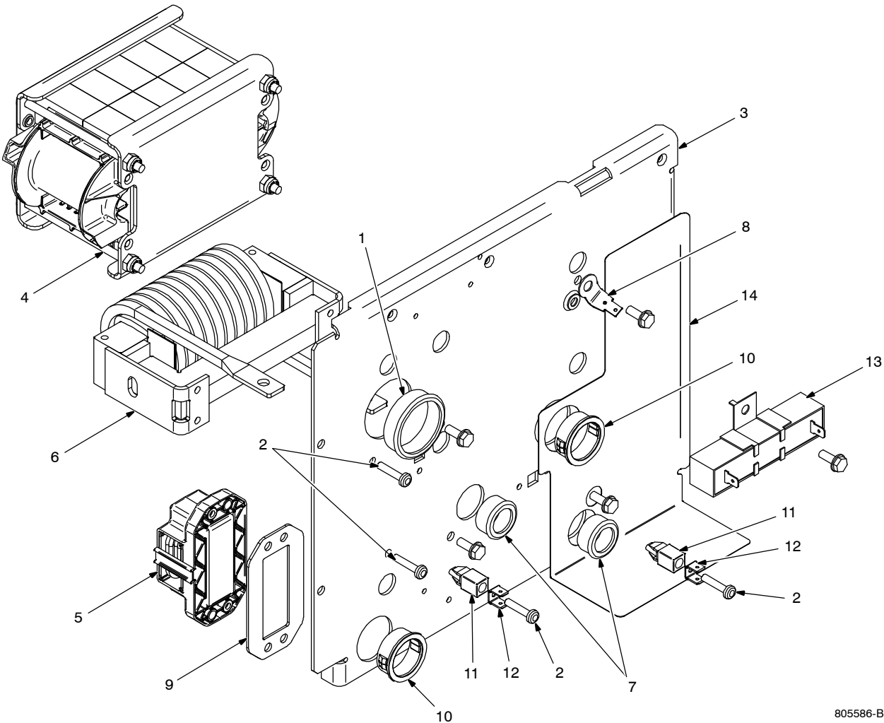
Figure 2-6. Wind Tunnel, Left Hand w/Components
