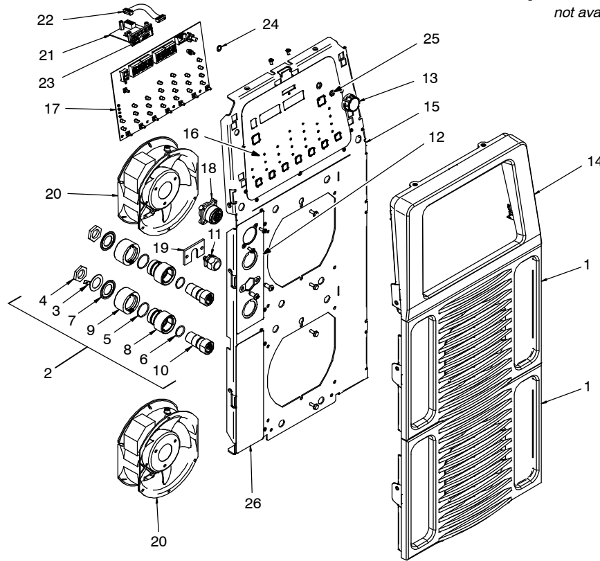
Figure 2-2. Panel, Front w/Components
