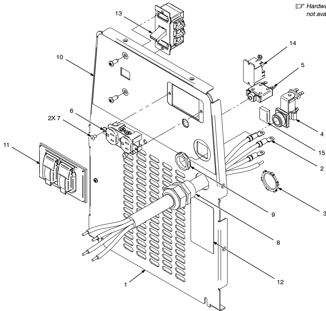
Figure 1-3. Panel, Rear w/Components
