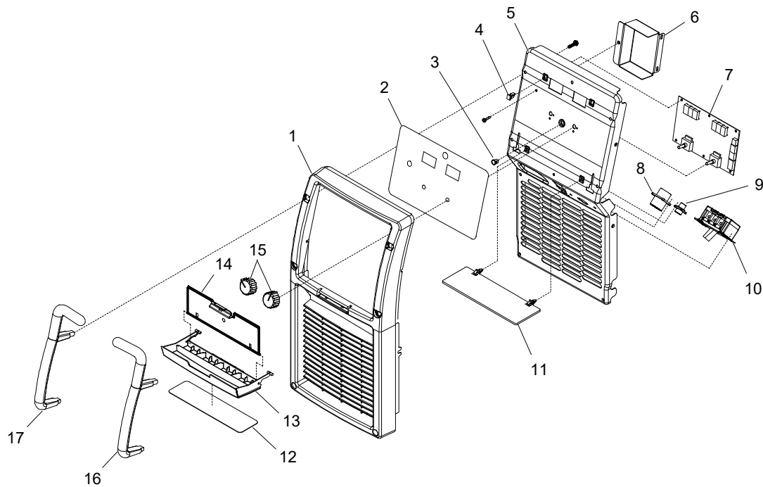
Panel, Front with Components
