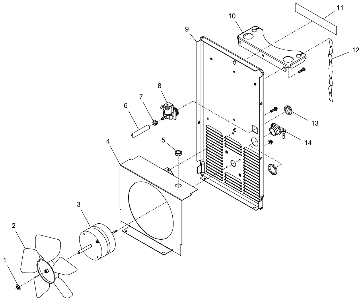
Panel, Rear with Components
