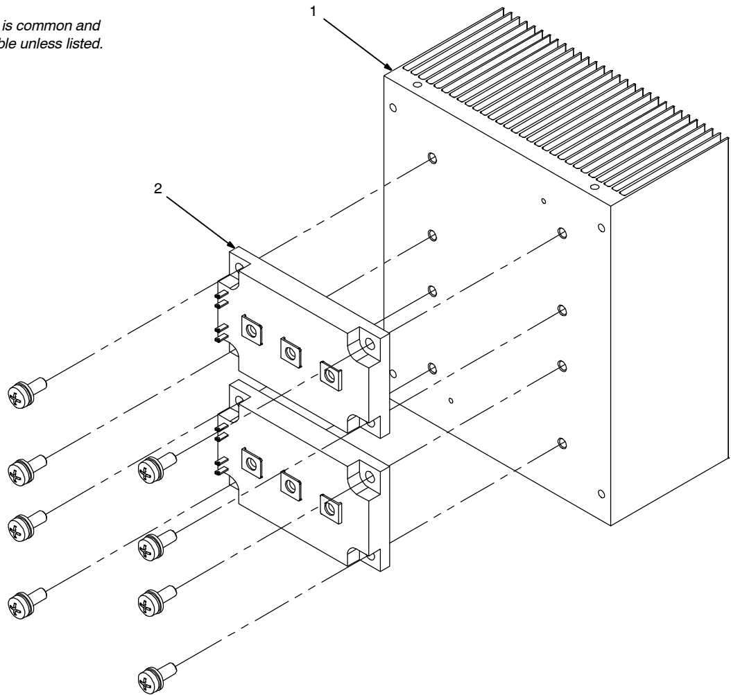
Figure 1-8. IGBT Heat Sink Assembly (Primary)
