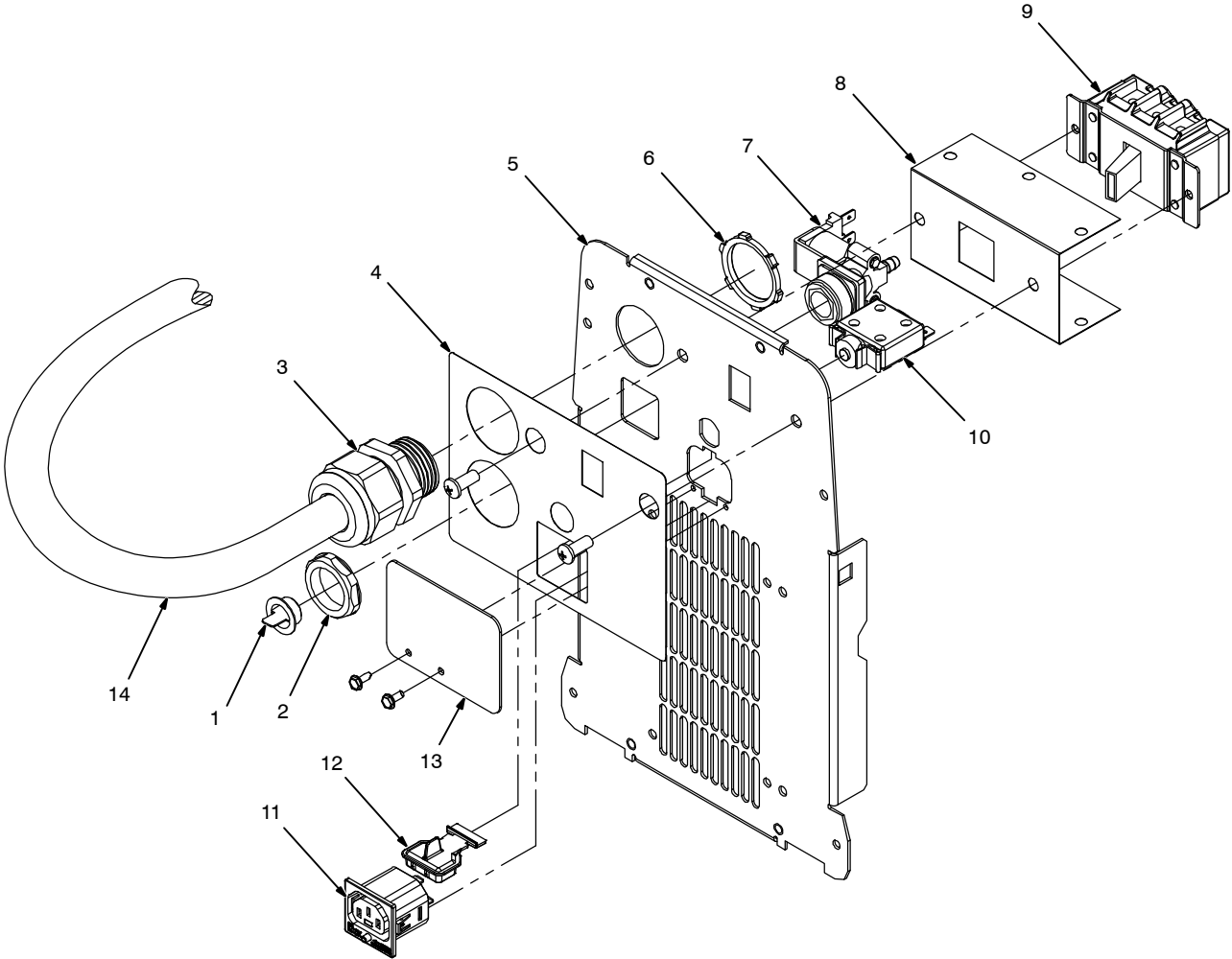
Figure 1-4. Panel, Rear w/Components
