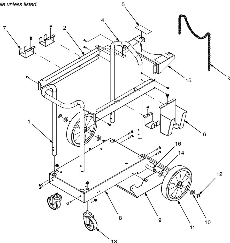
Figure 3-1. Complete Assembly For 254522
