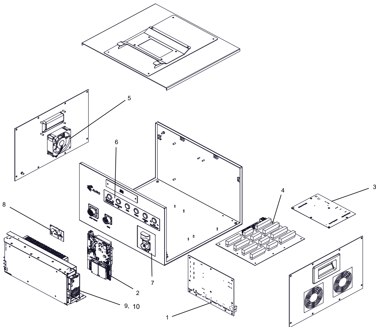
Control Box Assembly
