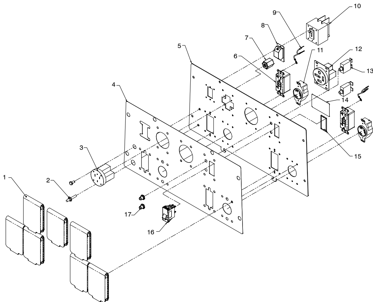
Figure 1-5. Panel, Auxiliary Power North America Prior To Serial No. ME260126E
