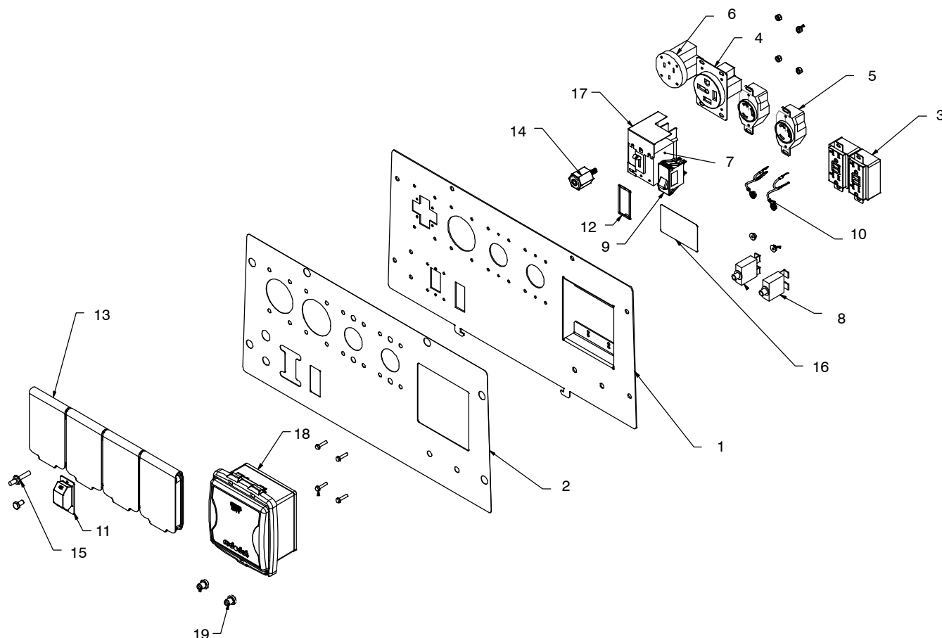
Figure 1-6. Panel, Auxiliary Power North America Eff w/Serial No. ME260126E
