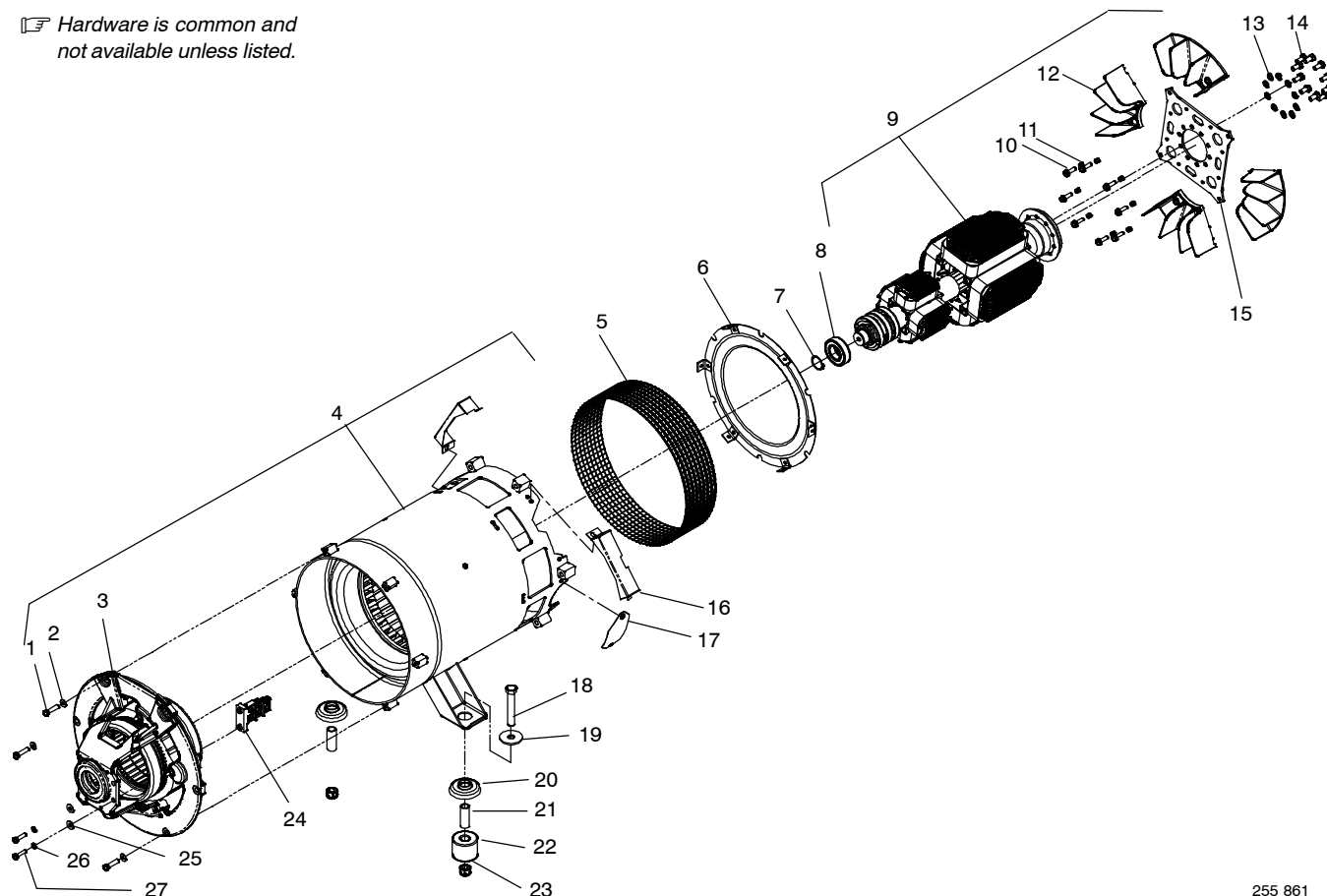
Figure 1-7. Generator
