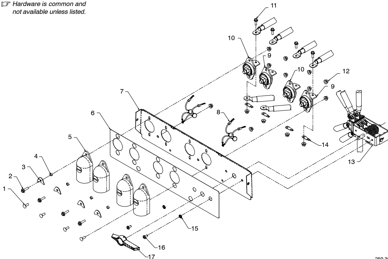
Figure 1-4. Panel, Weld Output
