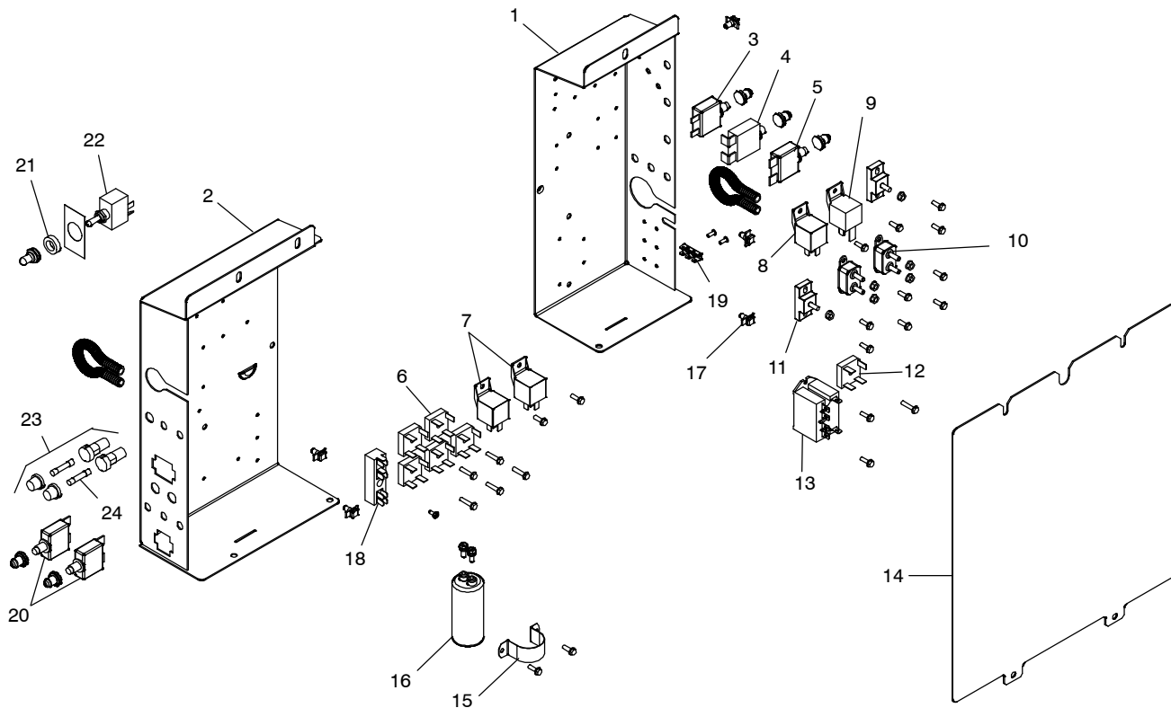
Figure 1-2. Control Box Assembly
