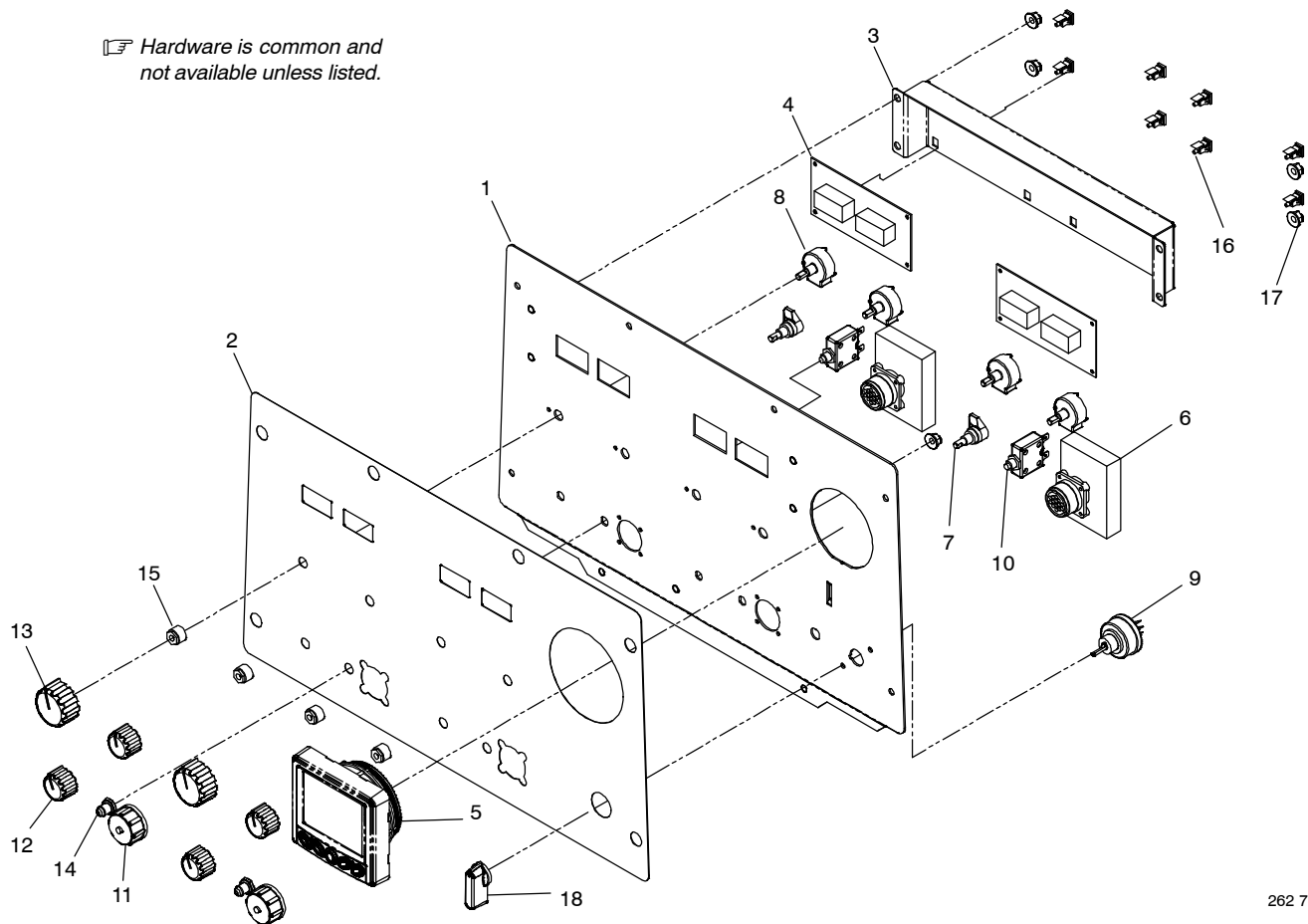
Figure 1-3. Panel, Front Engine & Weld Controls
