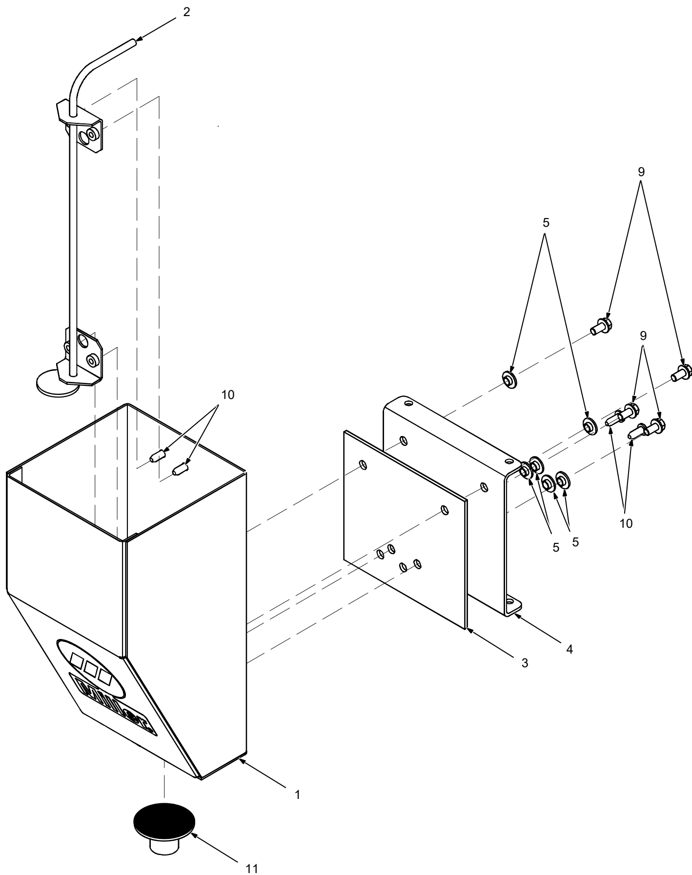
Manual Flux Hopper Main Assembly
