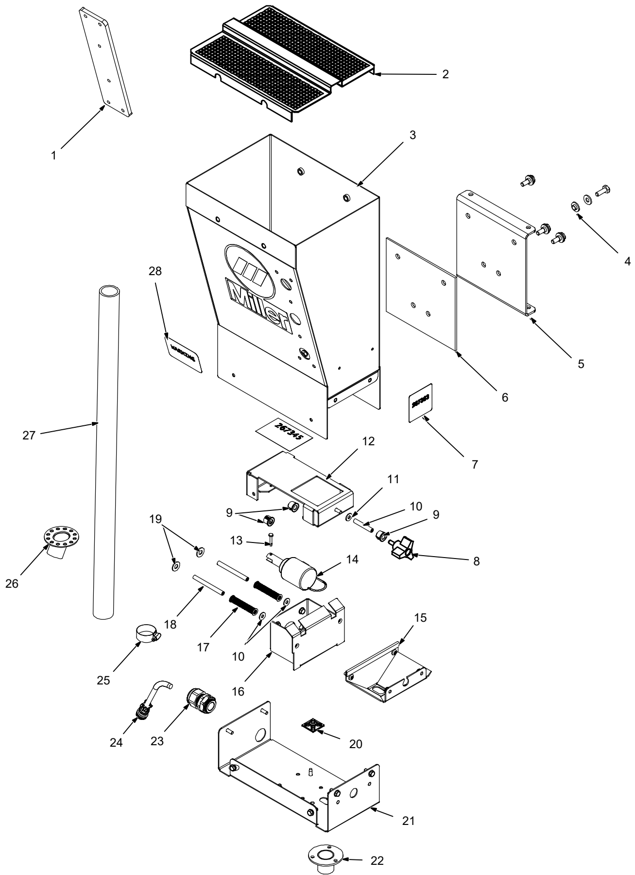
Flux Hopper Main Assembly
