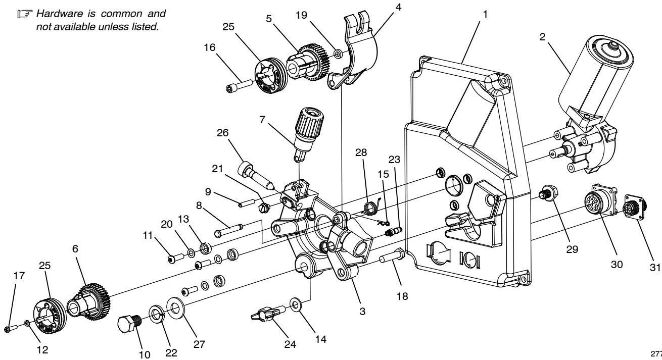
Figure 1-6. Wire Feed Drive Assembly (Figure 1-1, Item 6)
