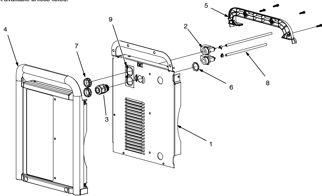
Figure 1-5. Rear Panel Assembly (Figure 1-1, Item 5)
