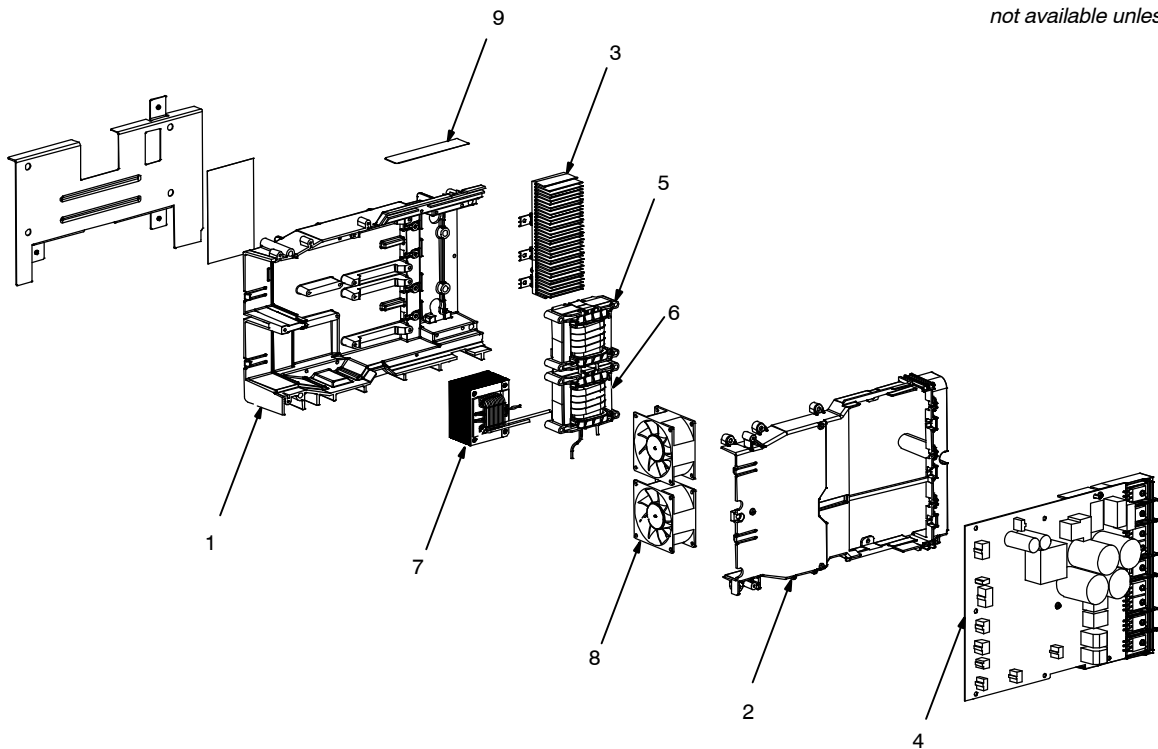
Figure 1-2. Windtunnel Assembly (Figure 1-1, Item 7)
