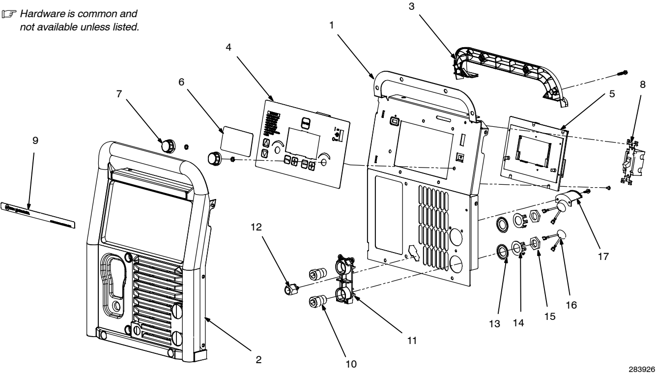
Figure 1-3. Front Panel Assembly (Figure 1-1, Item 4)
