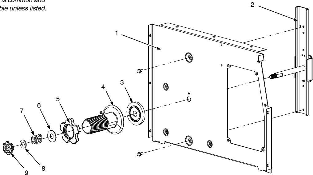
Figure 1-4. Center Baffle Assembly (Figure 1-1, Item 3)
