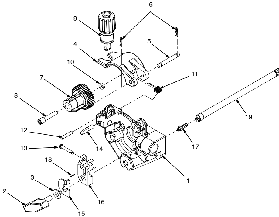
Figure 11-4. Exploded View Of Wire Drive Housing Assembly
