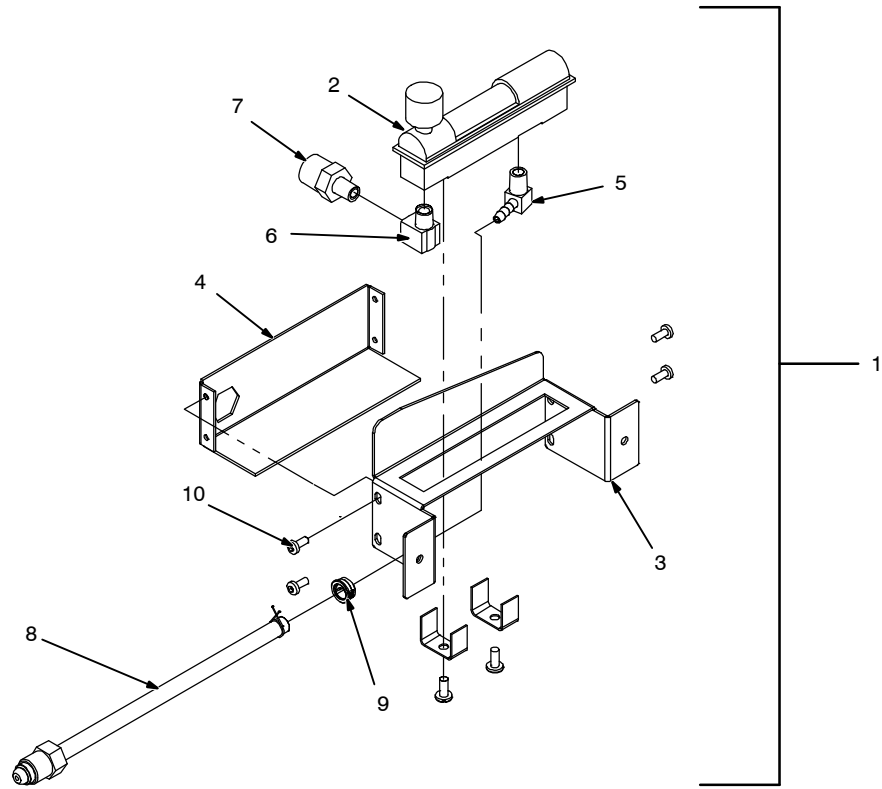
Figure 11-6. Optional Gas Flow Meter Kit
