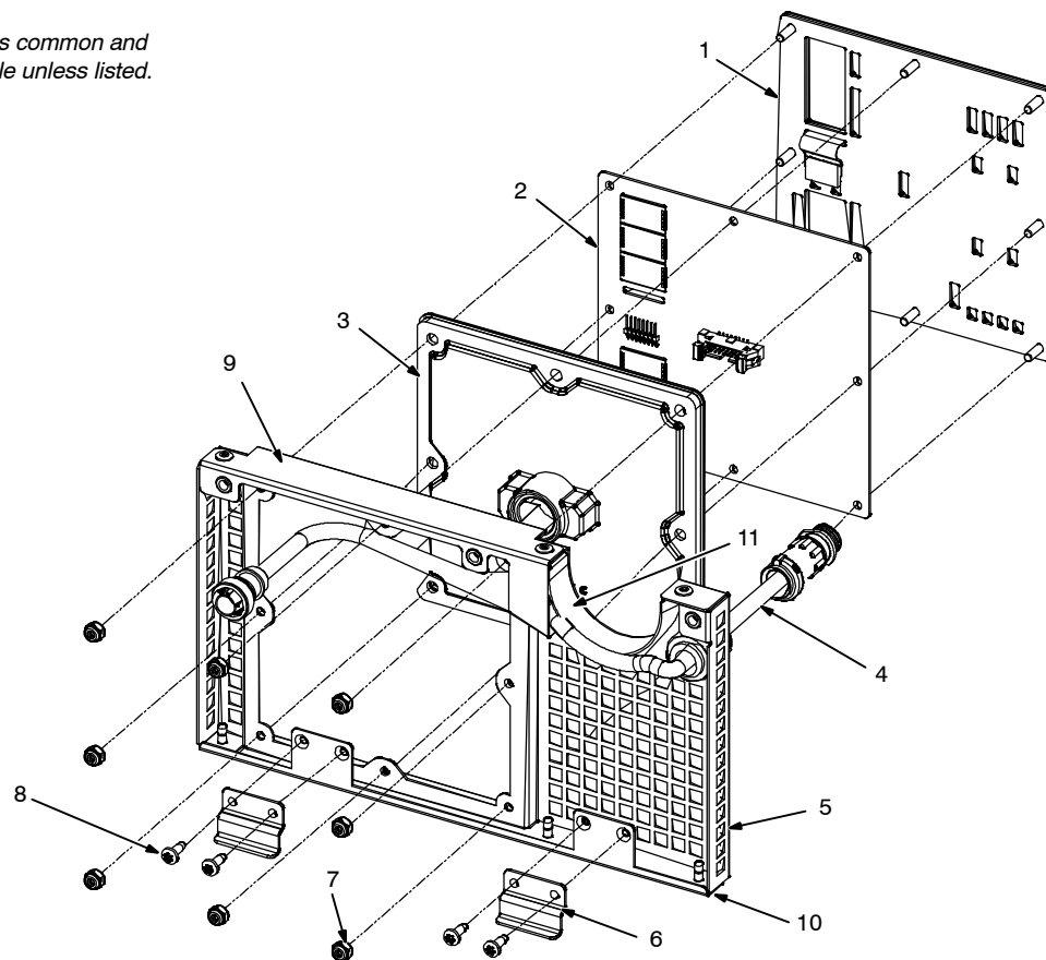
Figure 12-5. Exploded View Of User Interface External Assembly
