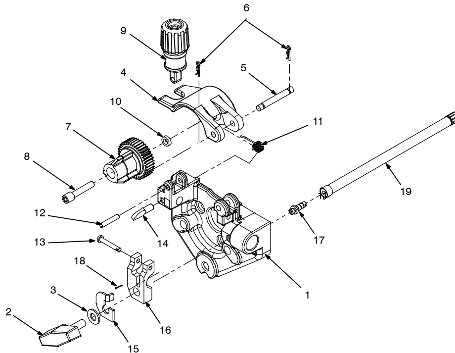
Figure 12-4. Exploded View Of Wire Drive Housing Assembly
