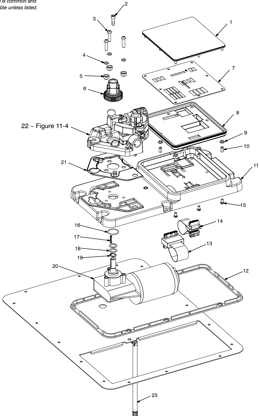
Figure 11-3. Exploded View Of Center Assembly
