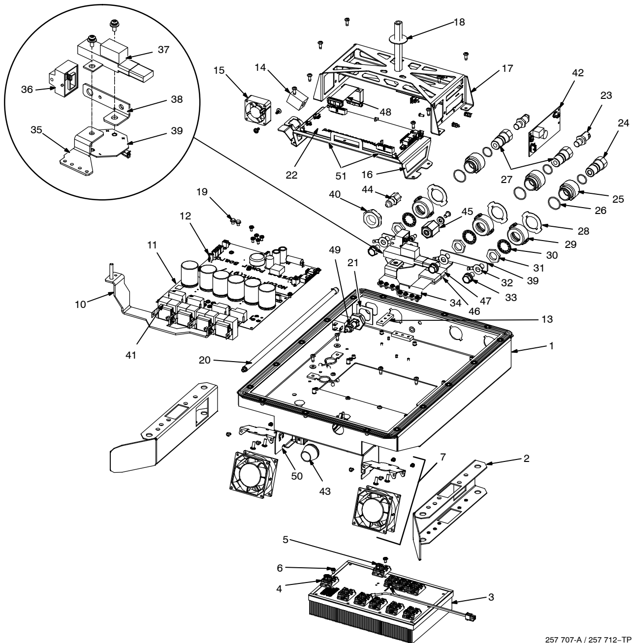
Figure 11-2. Exploded View Of Lower Chassis Assembly
