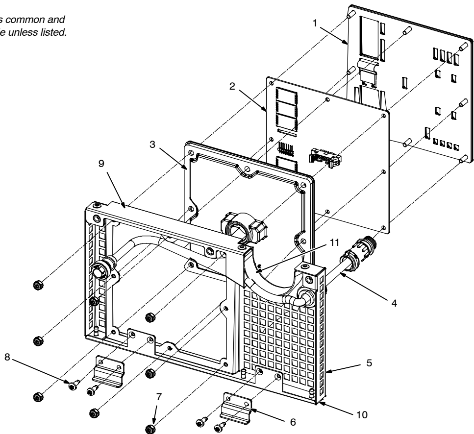
Figure 11-5. Exploded View Of User Interface External Assembly
