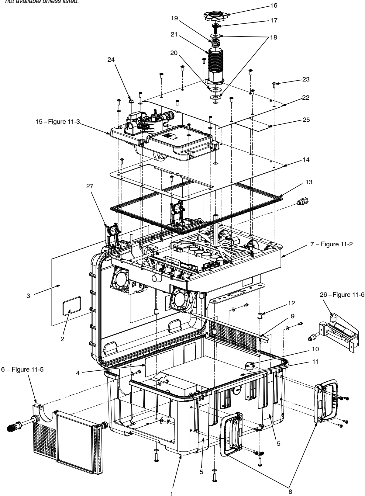
Figure 11-1. Exploded View Of Smart Feeder
