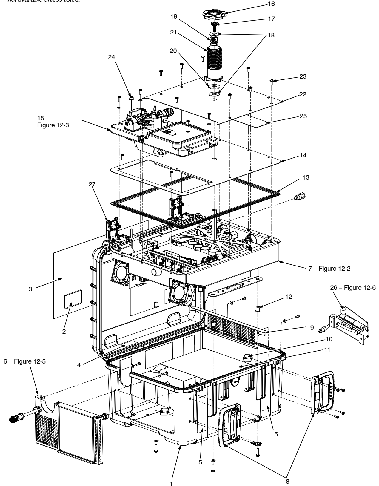
Figure 12-1. Exploded View Of Smart Feeder
