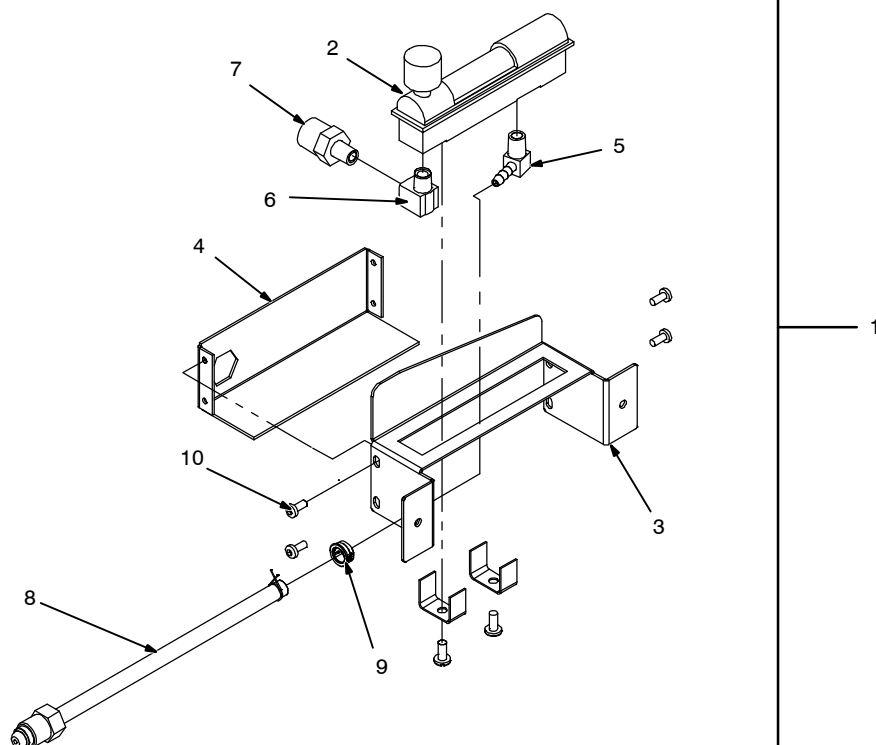
Figure 12-6. Optional Gas Flow Meter Kit
