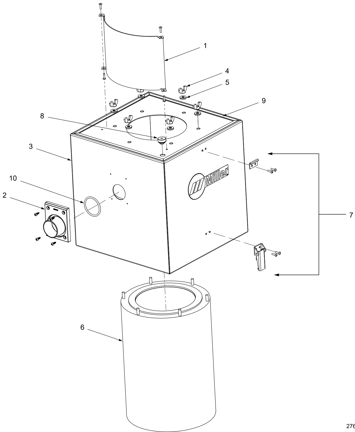
Filter Section Assembly
