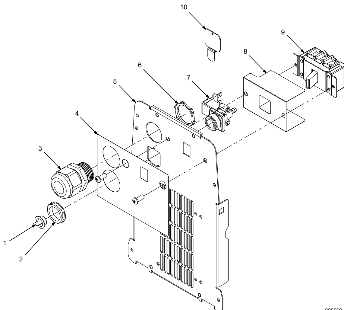
Panel, Rear with Components
