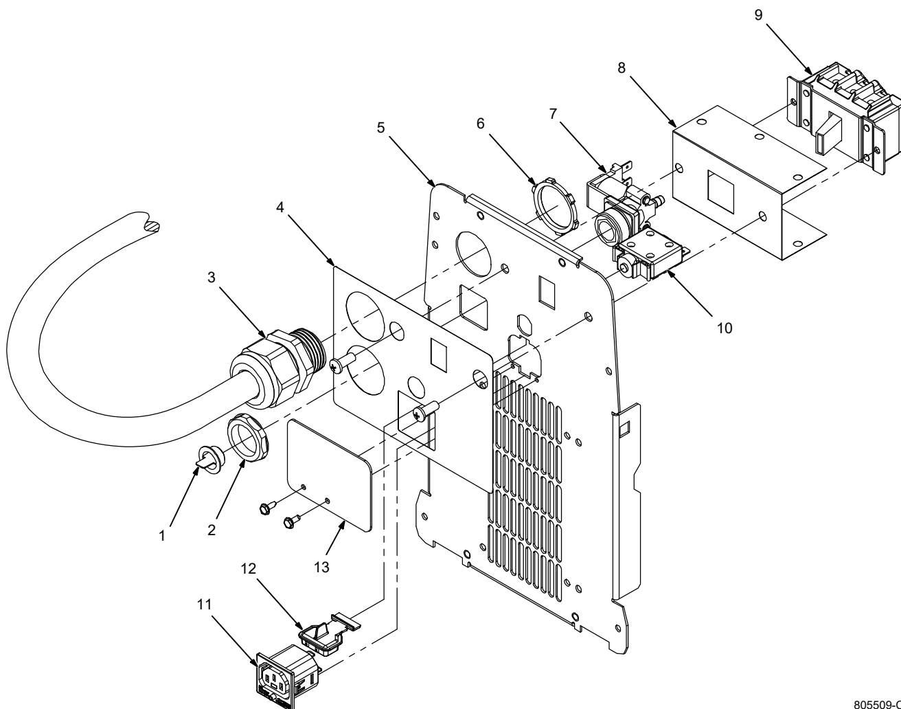
Panel, Rear with Components
