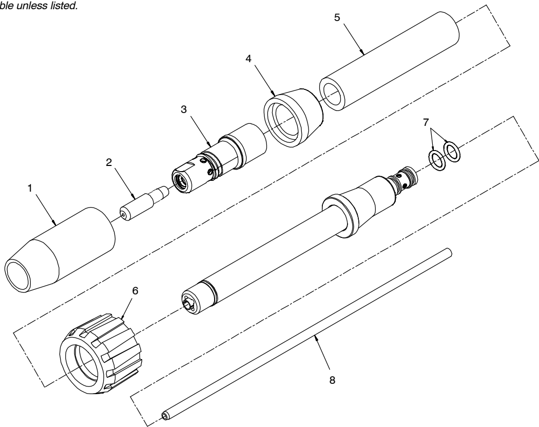
Figure 1-3. (Air) Head Tube Assembly Of XR - Pistol - Pro Gun
