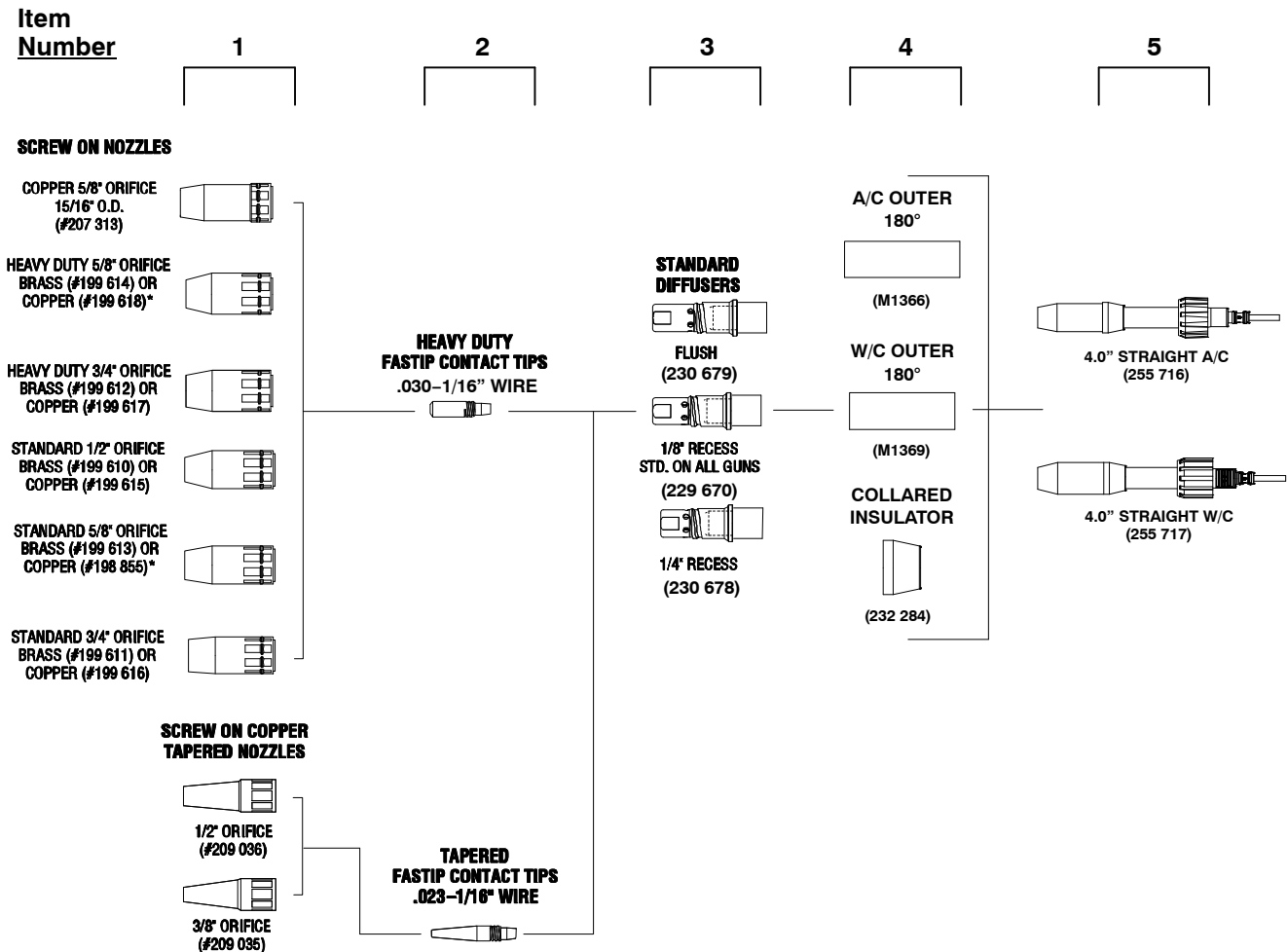
Figure 2-1. Consumables Flowchart
