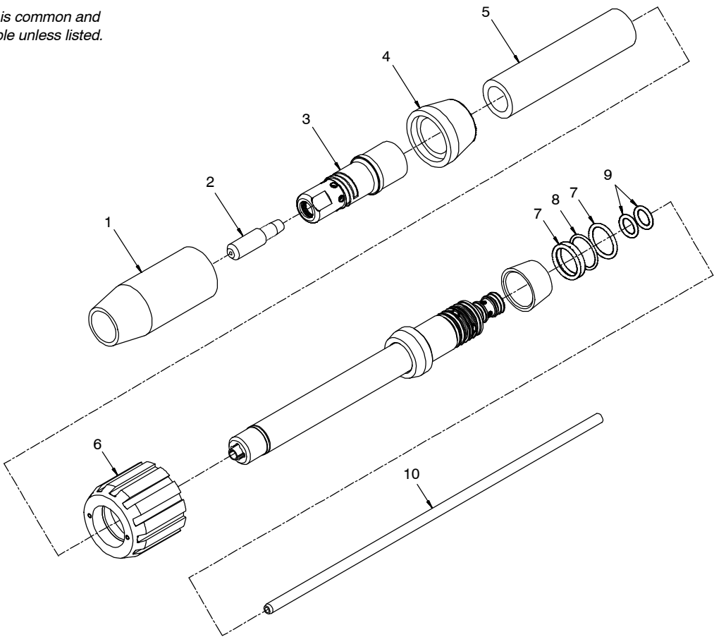
Figure 1-2. (Water) Head Tube Assembly Of XR - Pistol - Pro Gun
