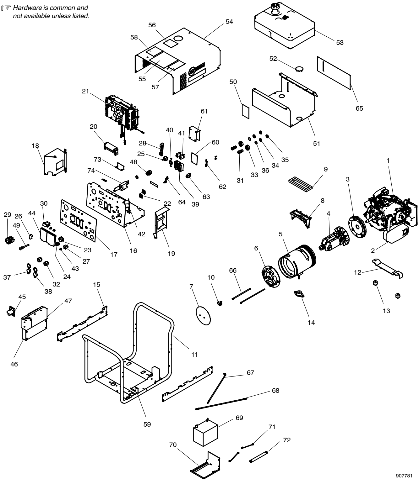
Figure 1-1. Main Assembly
