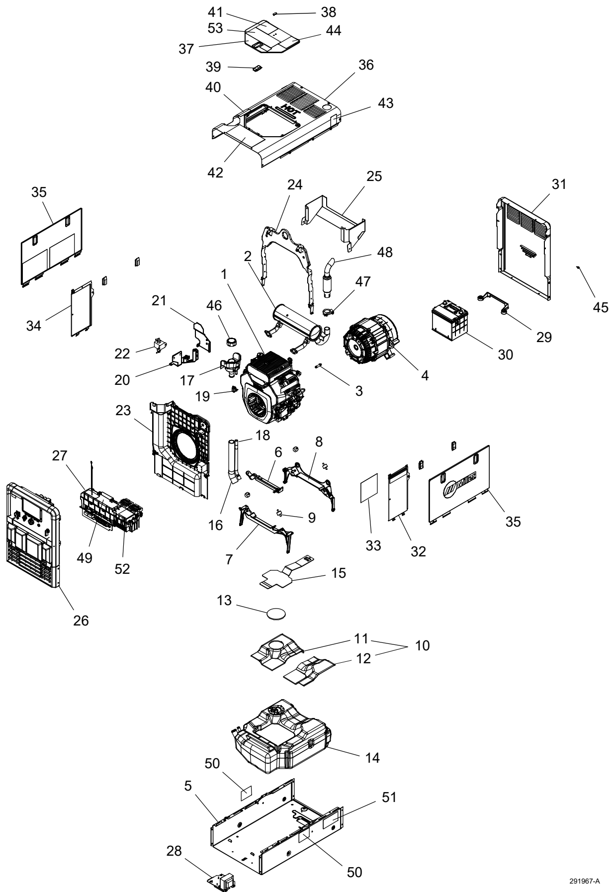
Main Assembly
