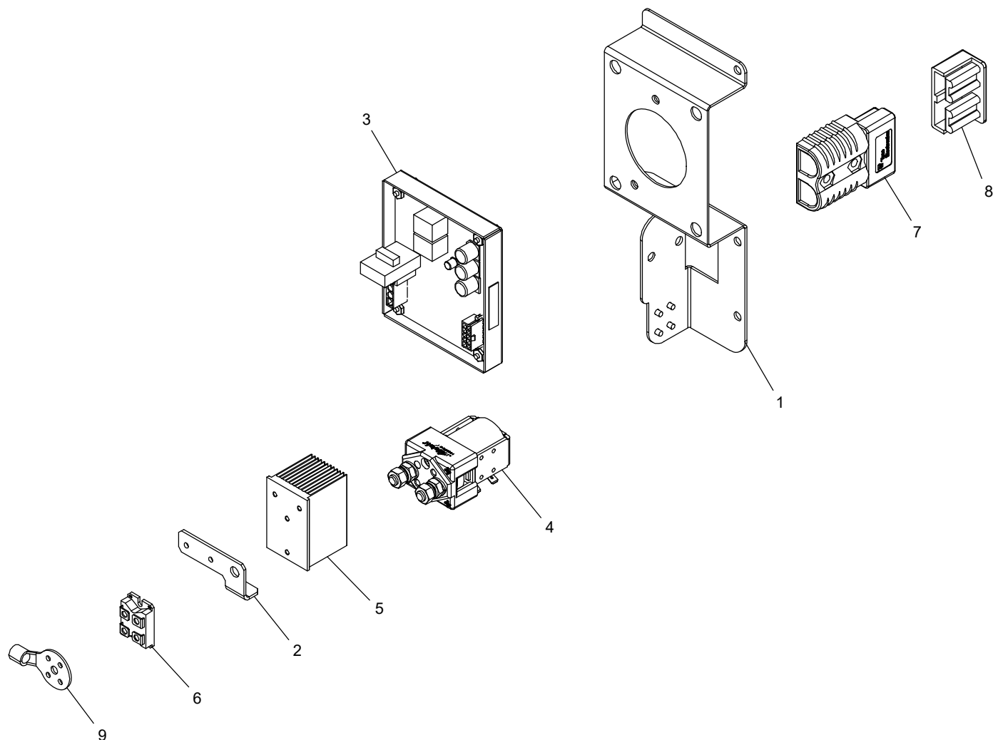
Battery Charge Assembly (293620)
