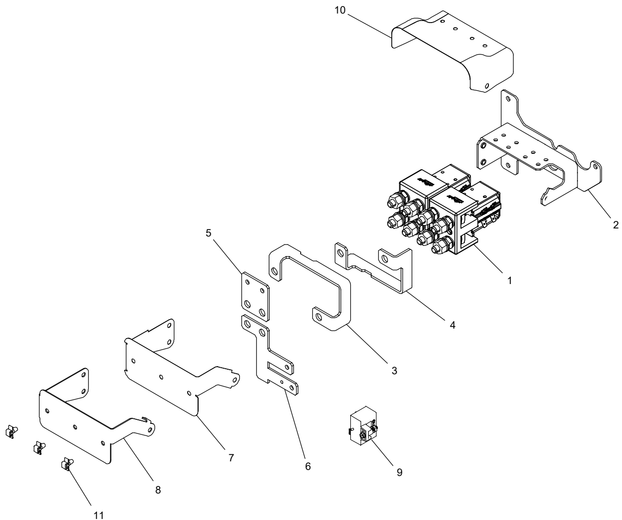
Reverse Polarity Assembly (289198)
