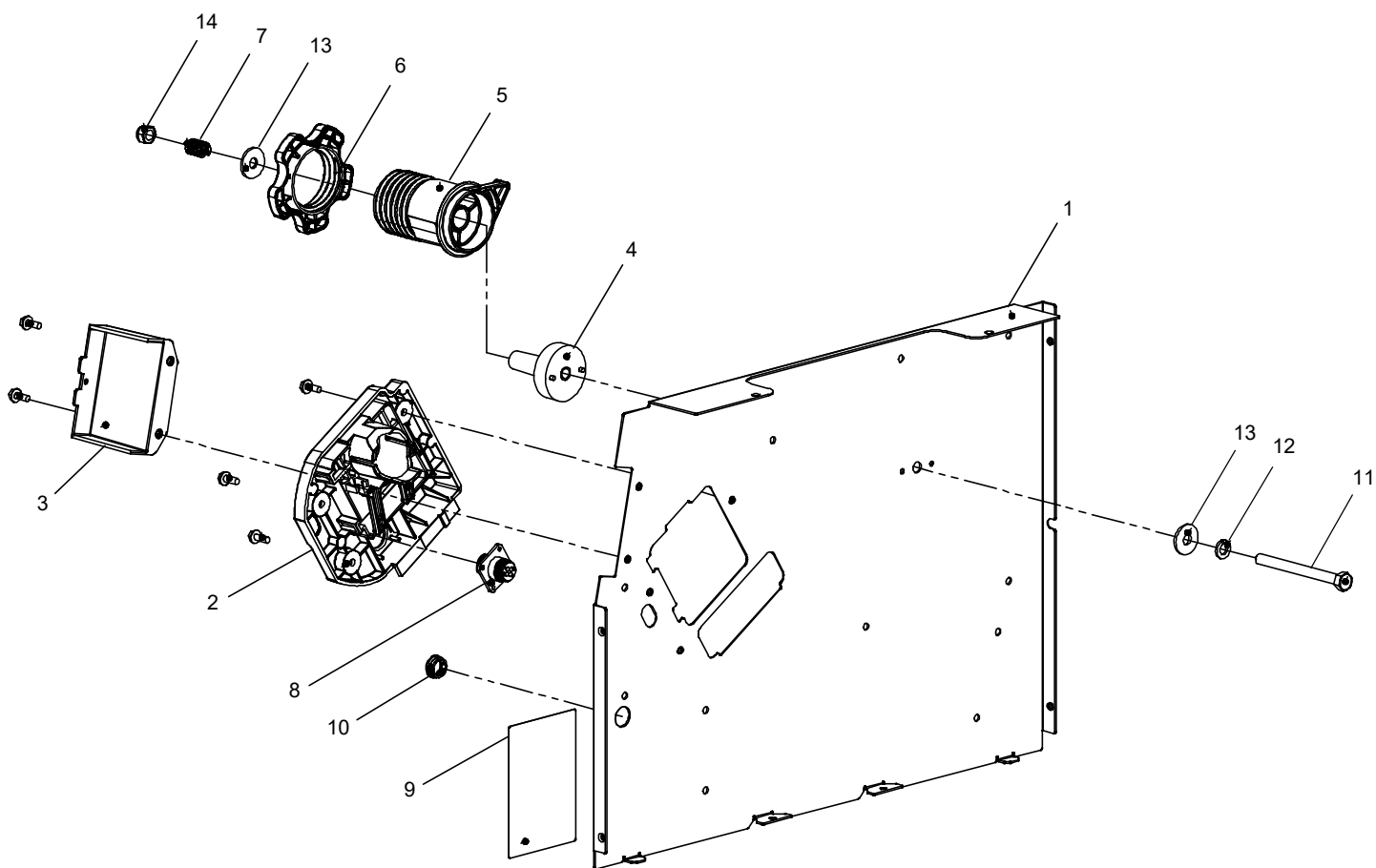
Baffle Assembly
