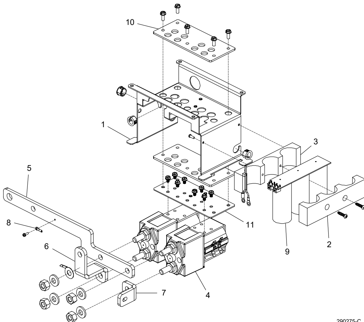
Contactor Panel Assembly
