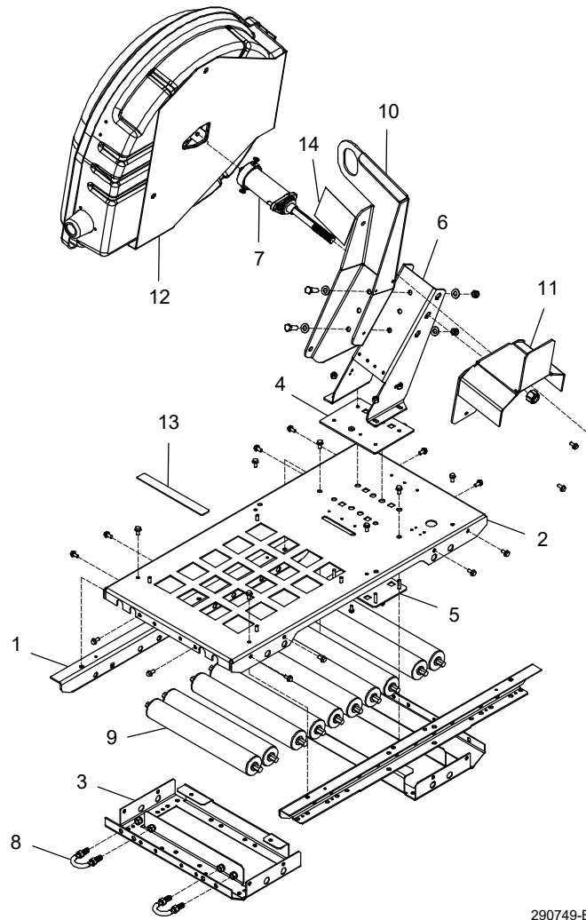
Base, Sled Assembly with Rollers
