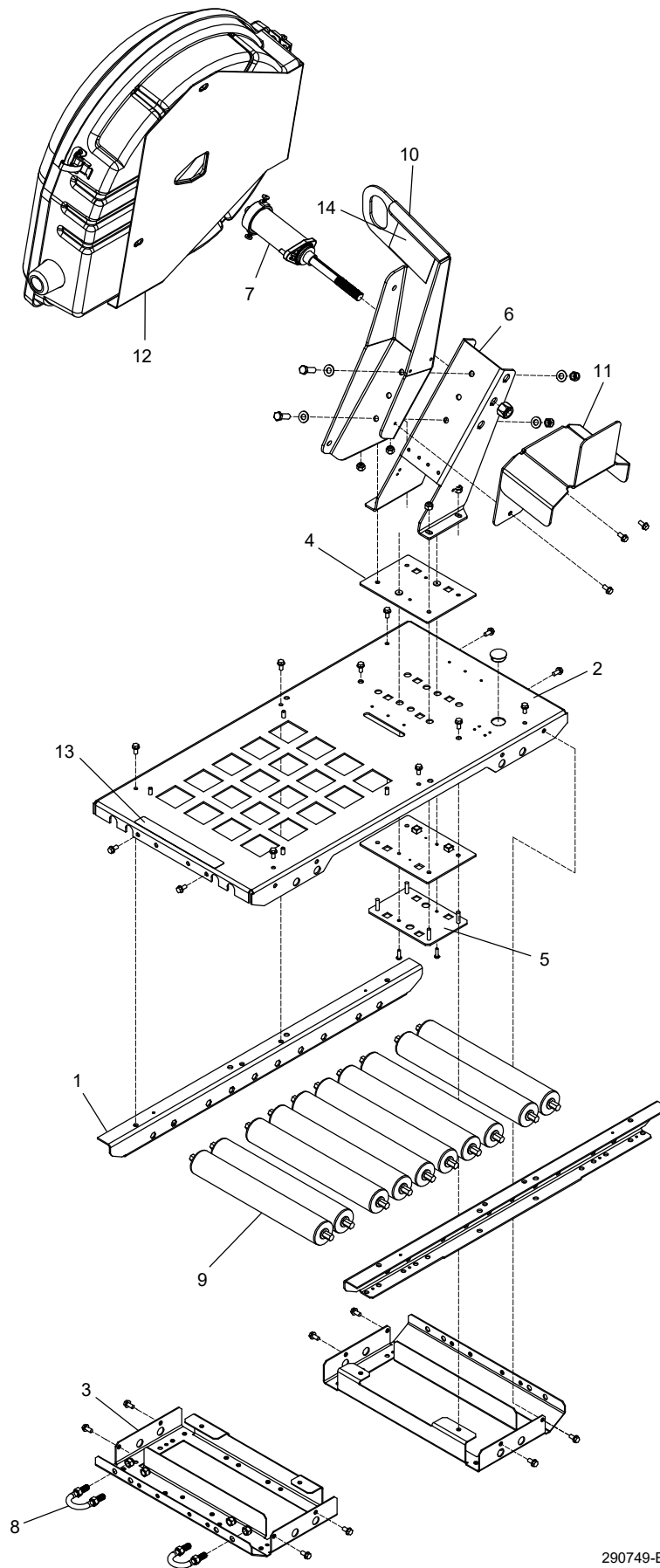
Base, Sled Assembly with Rollers
