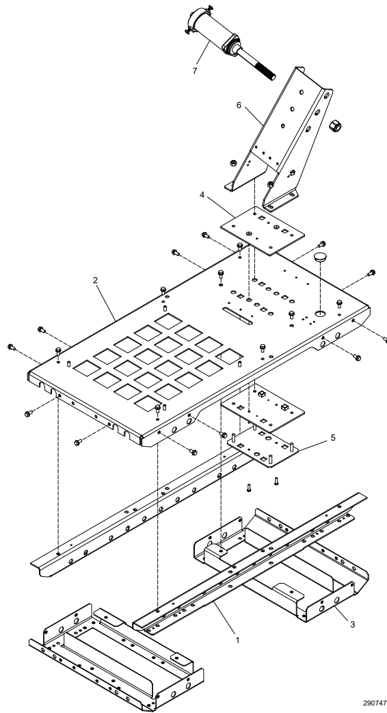
Base, Sled Assembly with Rails
