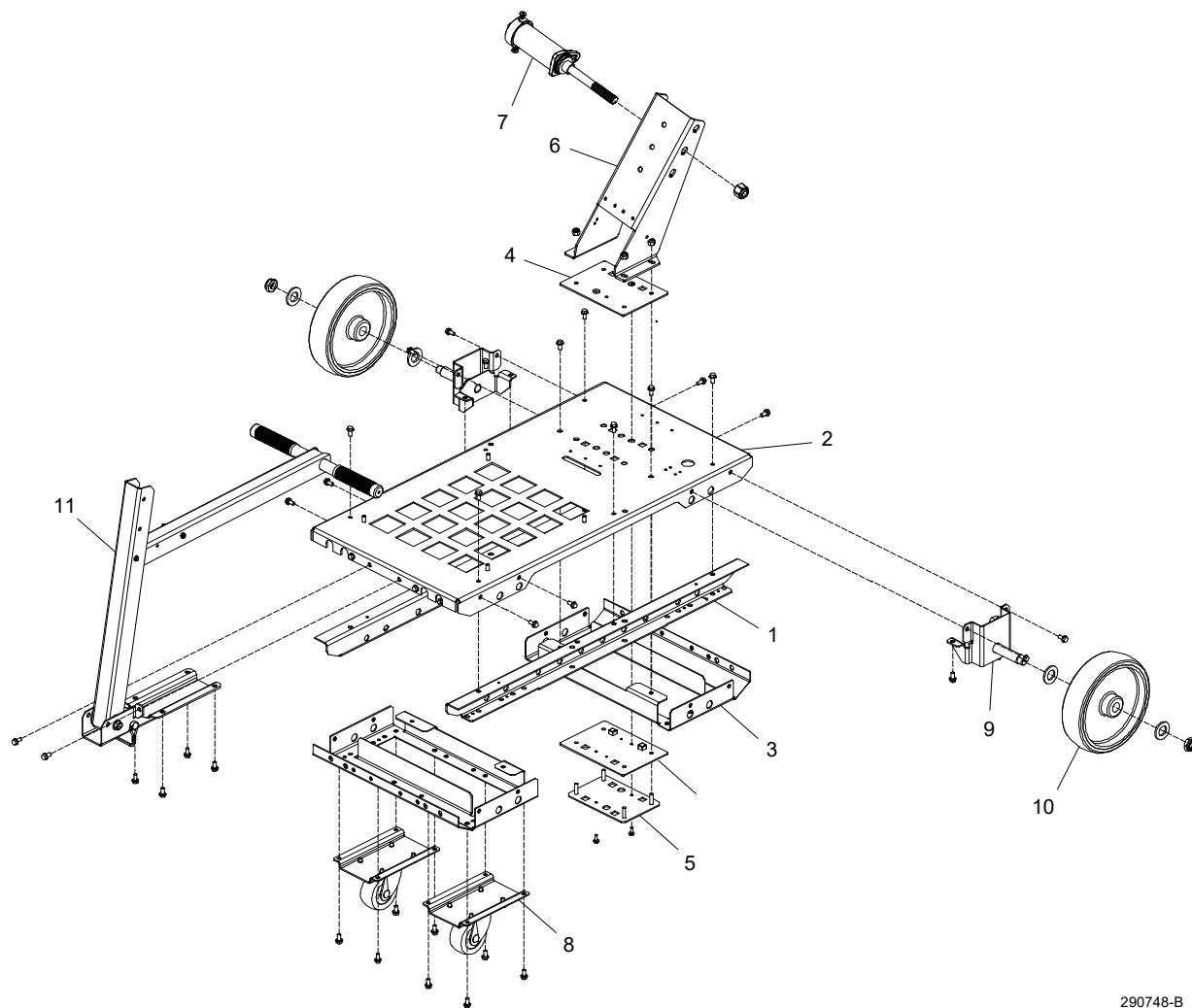
Base, Sled Assembly with Wheels
