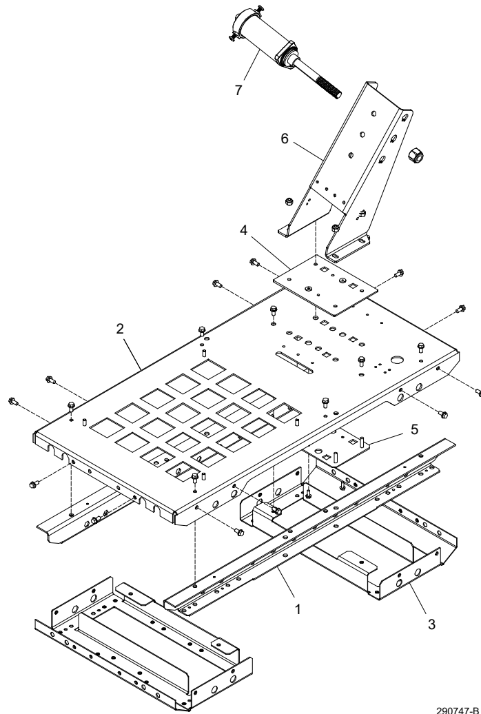
Base, Sled Assembly with Rails
