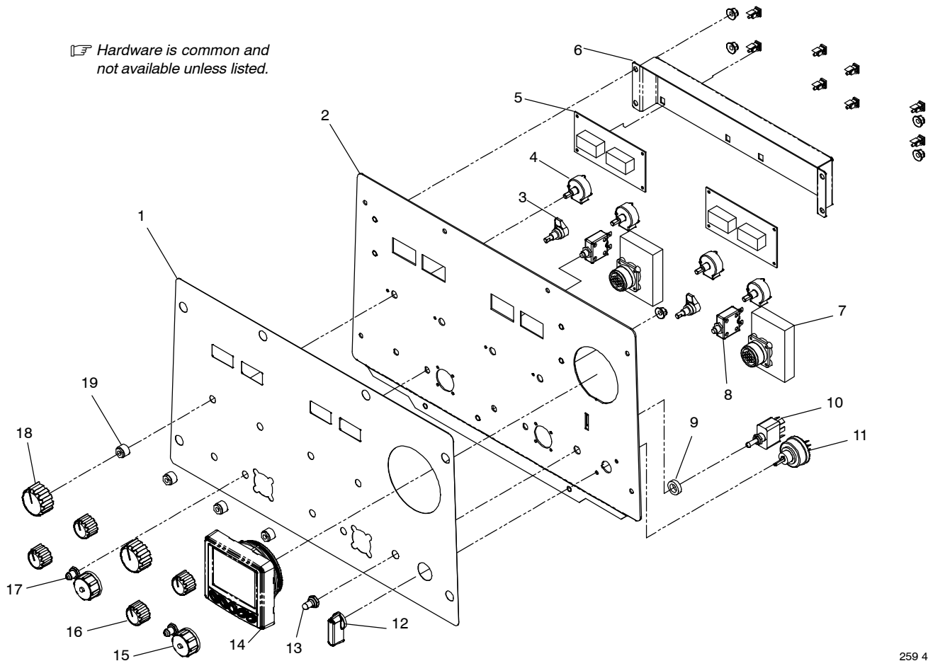
Figure 1-3. Panel, Front Engine & Weld Controls
