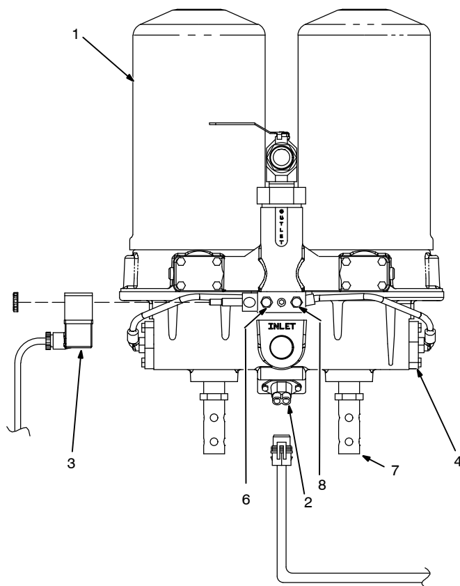
Figure 1-9. Optional Air Dryer Assemblies
