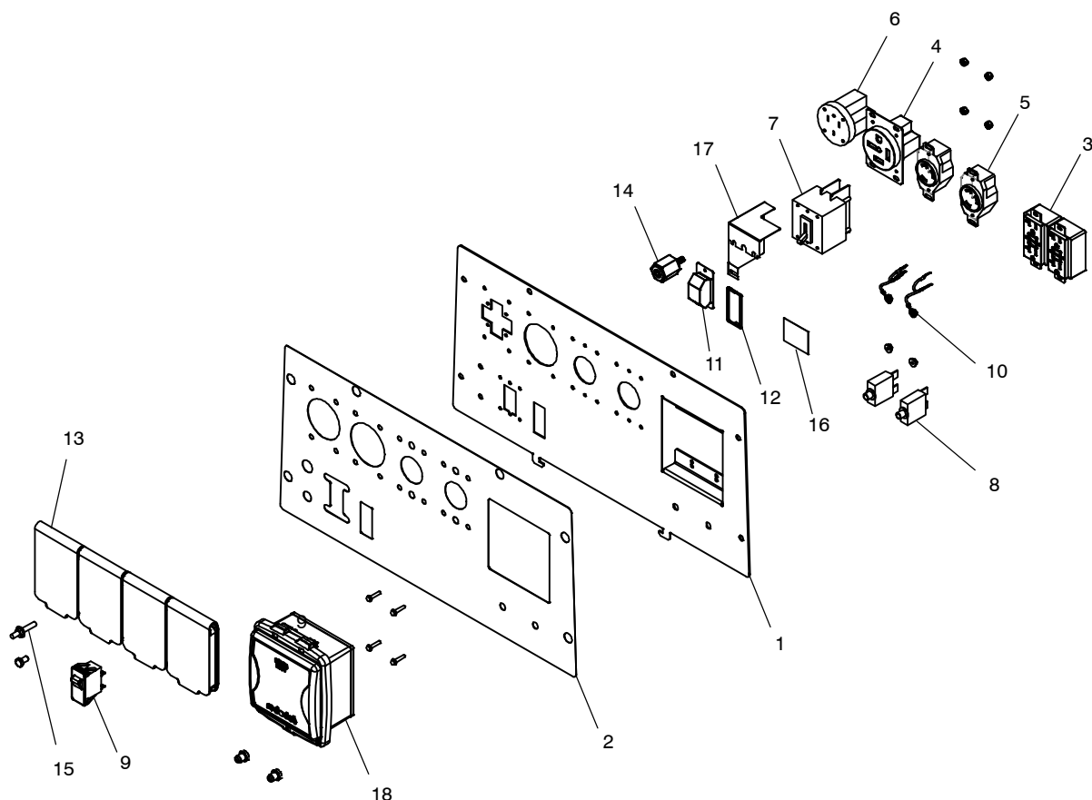
Figure 1-6. Panel, Auxiliary Power North America (Eff w/Serial No. ME260126E)
