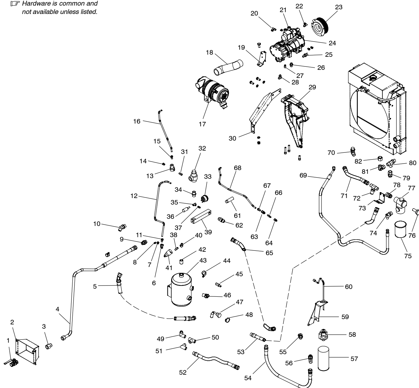
Figure 1-8. Air Compressor
