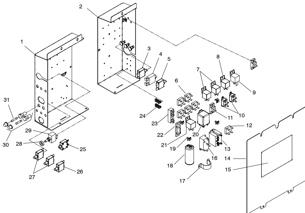
Figure 1-2. Control Box Assembly
