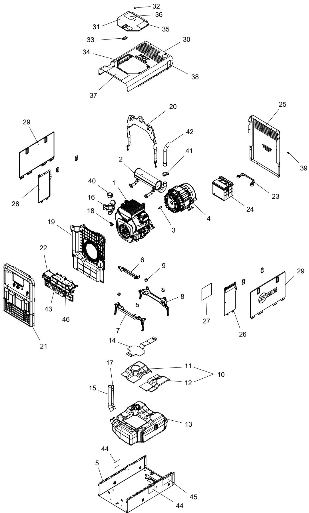
Main Assembly
