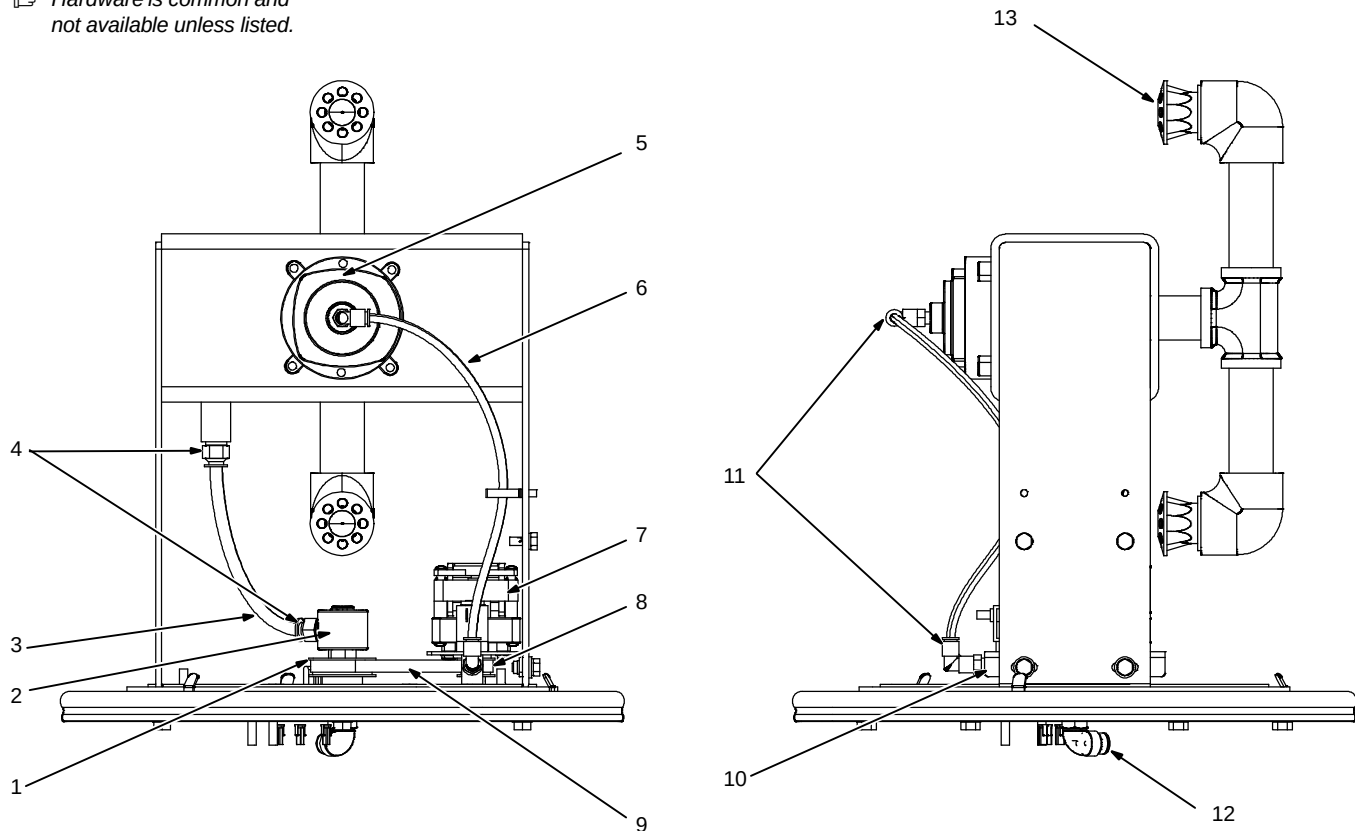
Figure 10-3. Self-Cleaning Assembly
