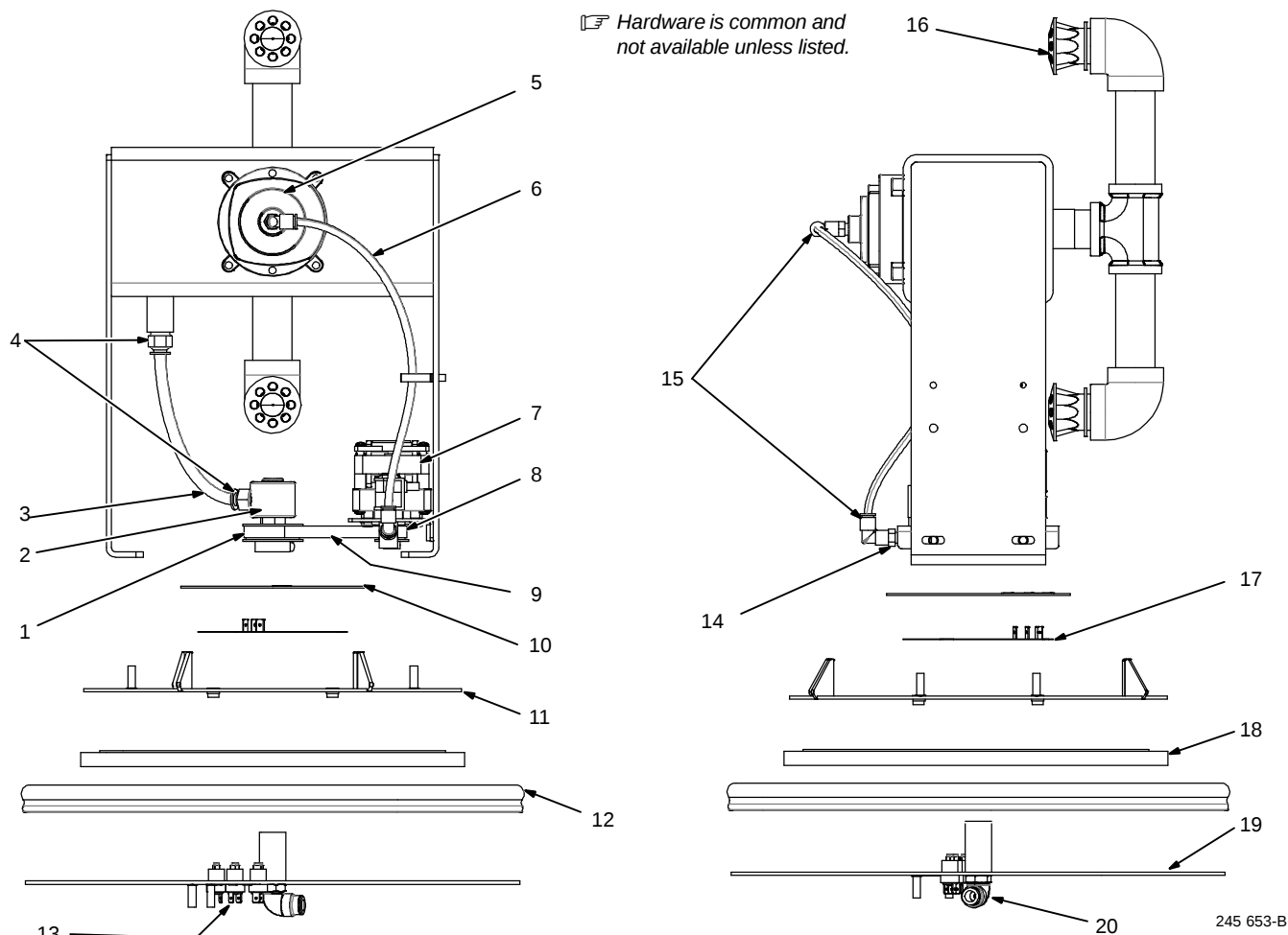
Figure 10-3. Self-Cleaning Assembly
