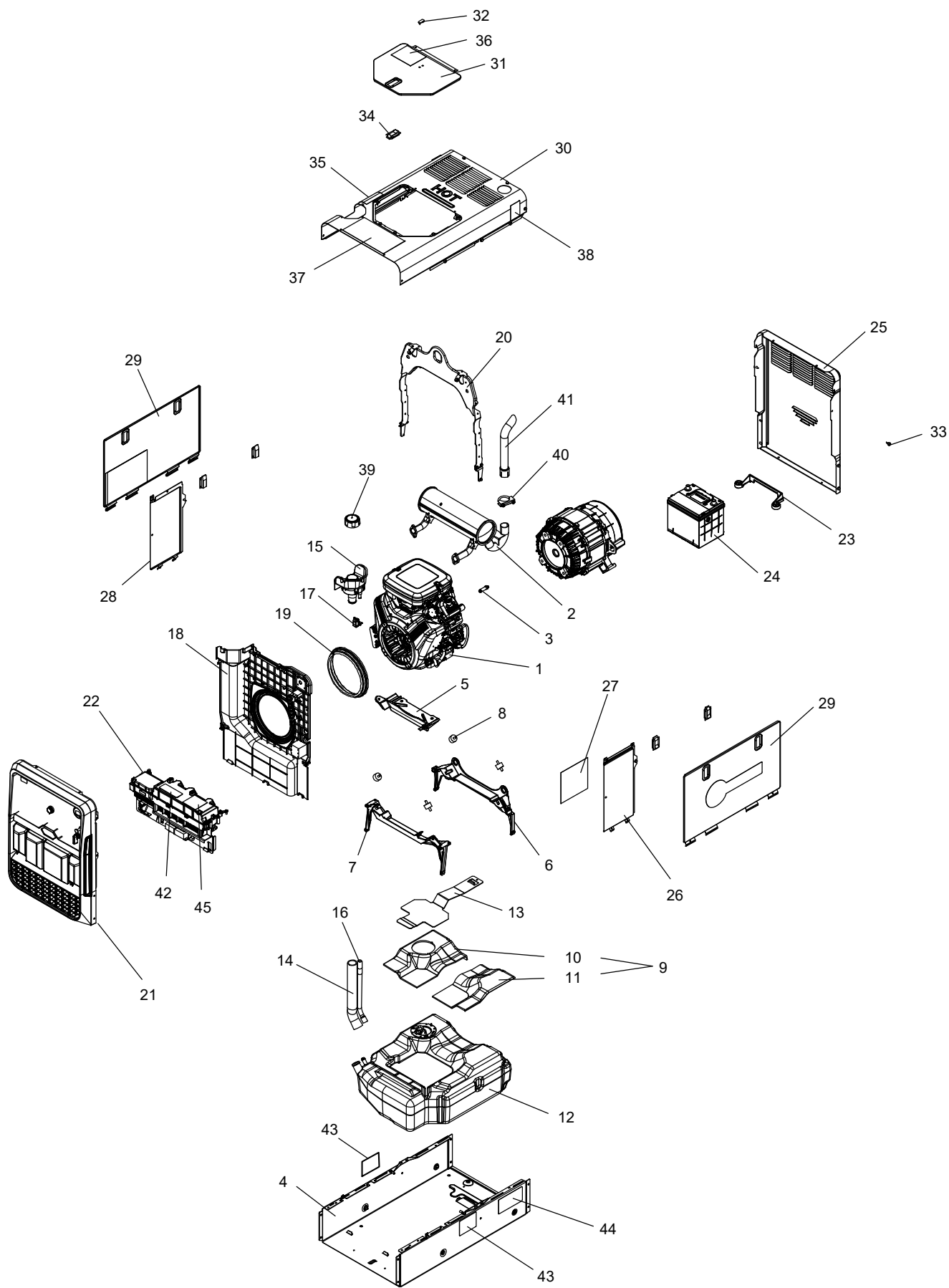
Main Assembly
