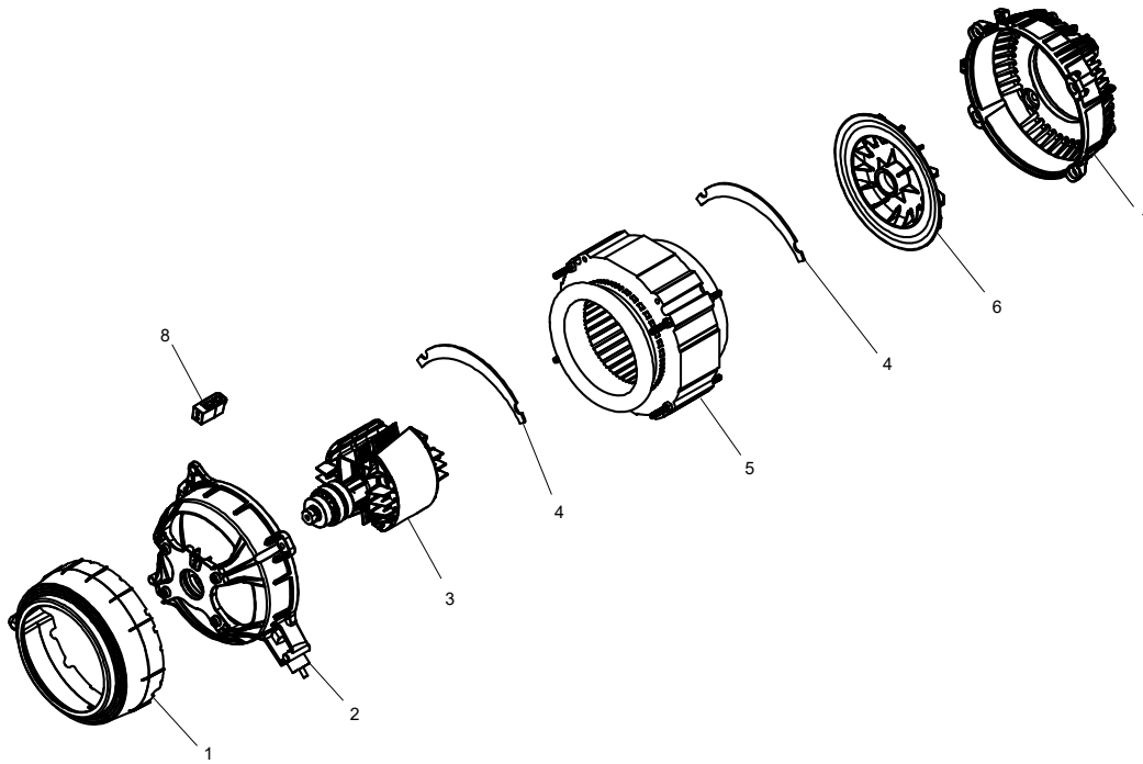
Generator Assembly
